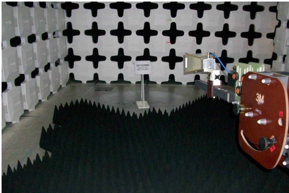
Horn Antenna – 1GHz to 18GHz
