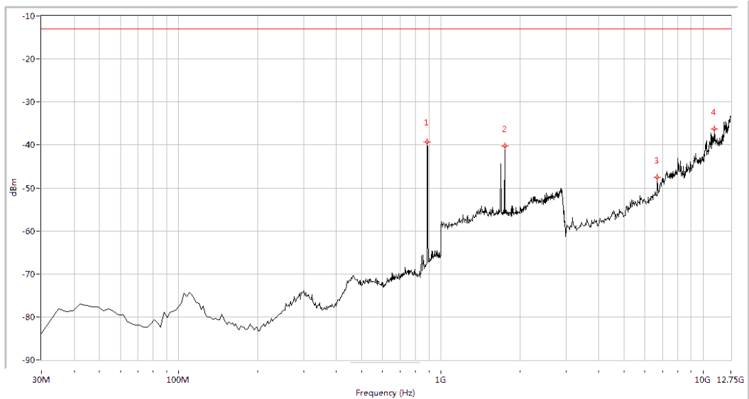
(Plot C.5: WCDMA 850MHz Channel = 4233, Test Antenna Horizontal)
