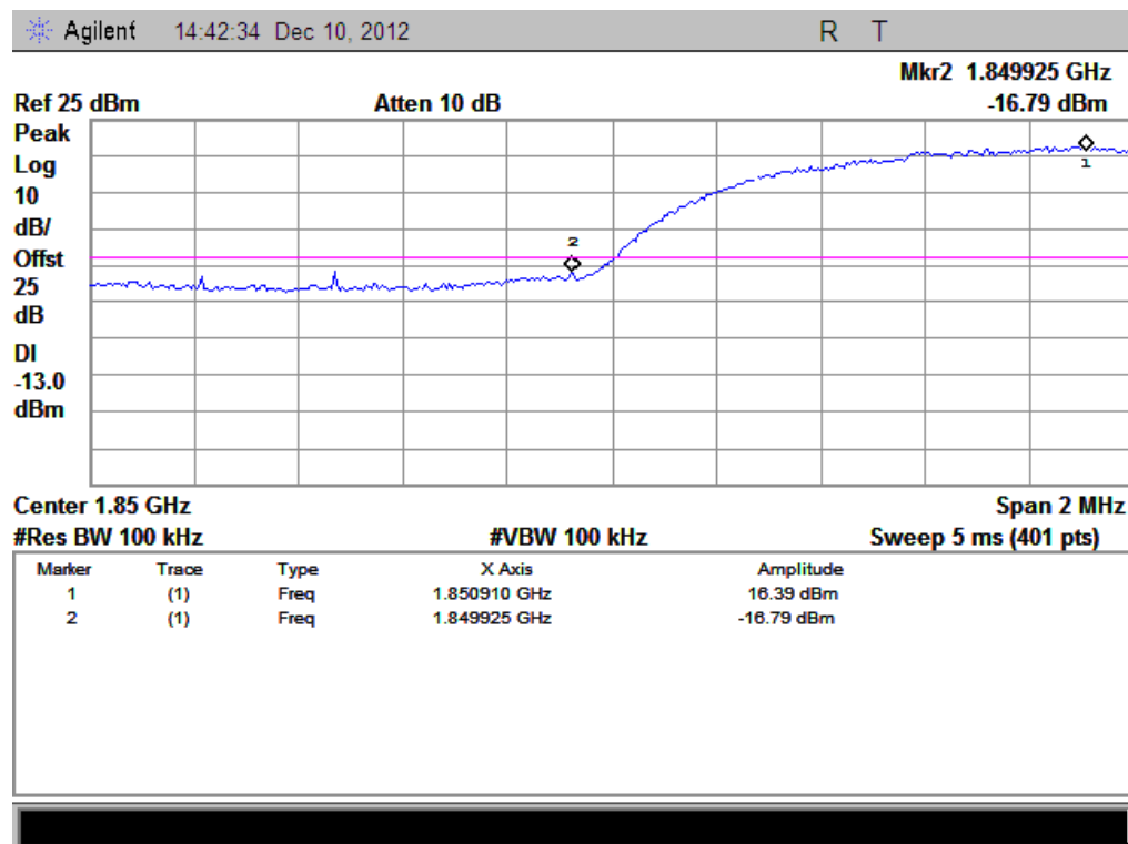
(Plot K: HSDPA1900 Channel = 9262)
