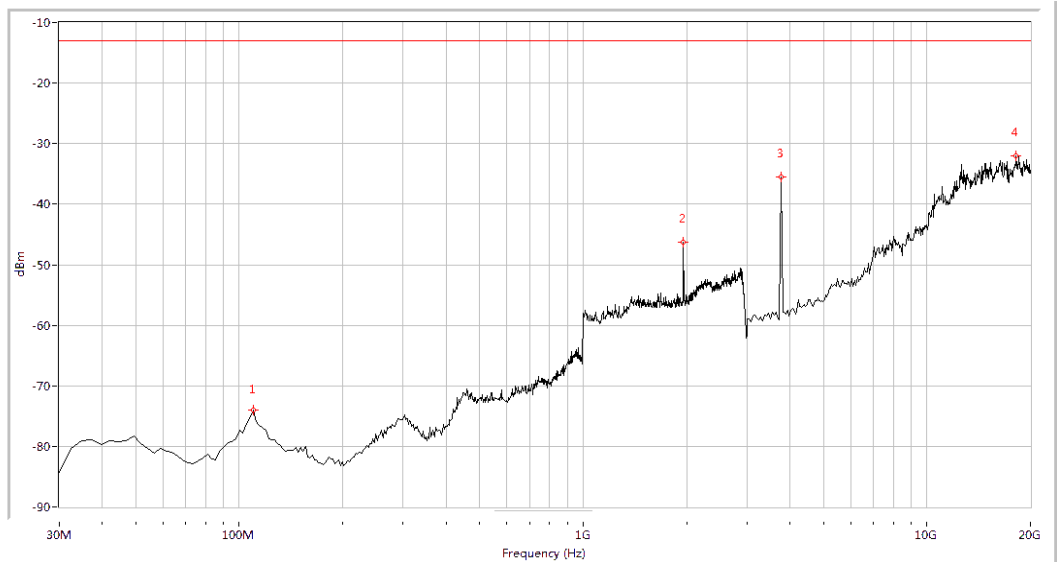
(Plot D.3: WCDMA 1900MHz Channel = 9400, Test Antenna Horizontal)
