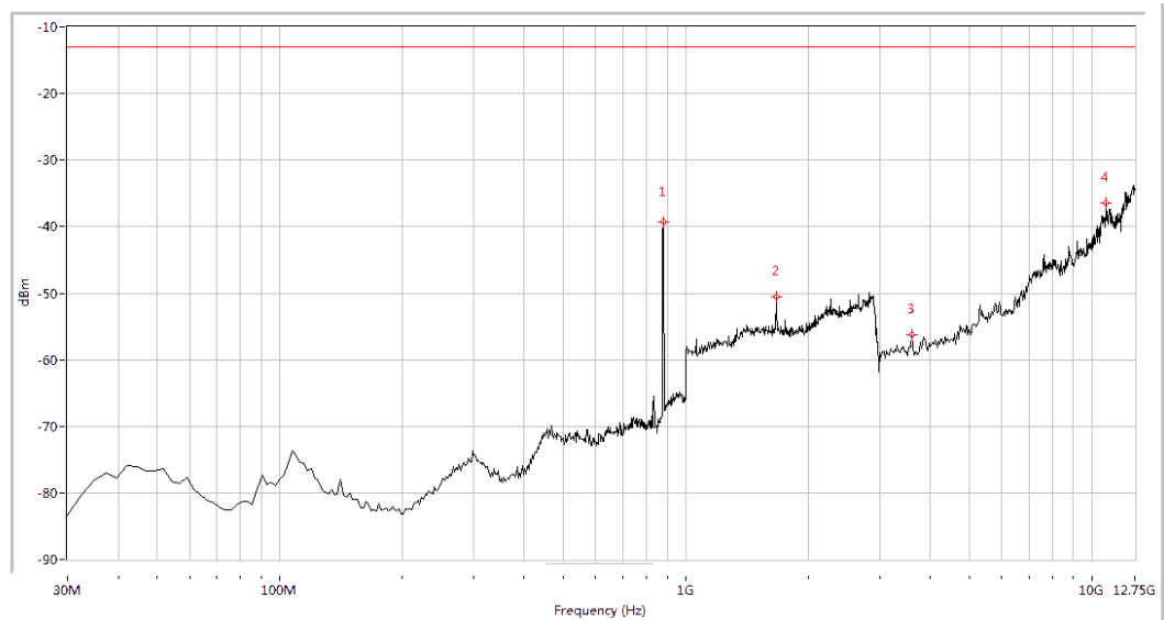
(Plot C.3: WCDMA 850MHz Channel = 4175, Test Antenna Horizontal)
