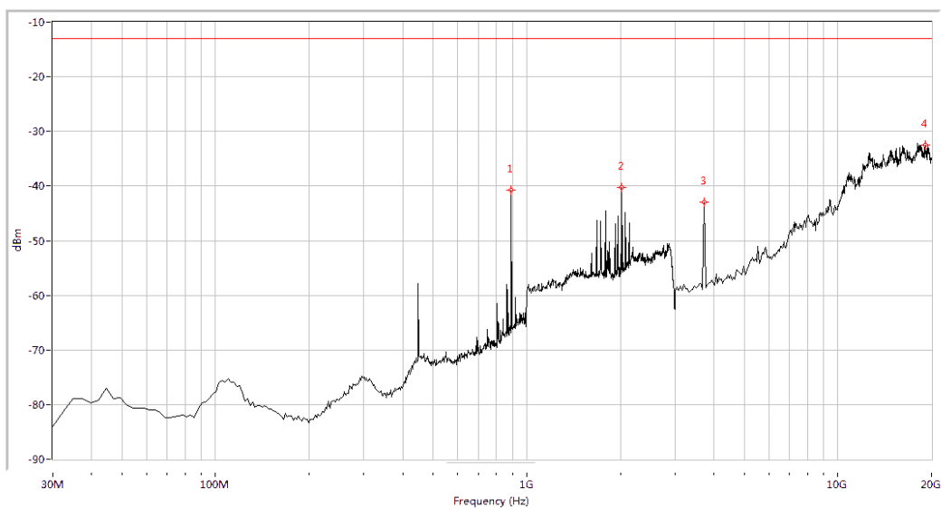
(Plot B.1: GSM 1900MHz Channel = 512, Test Antenna Horizontal)
