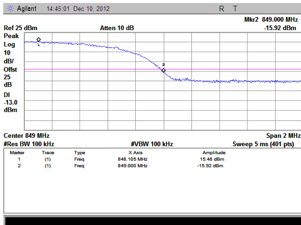
(Plot J: HSDPA 850 Channel = 4233)
