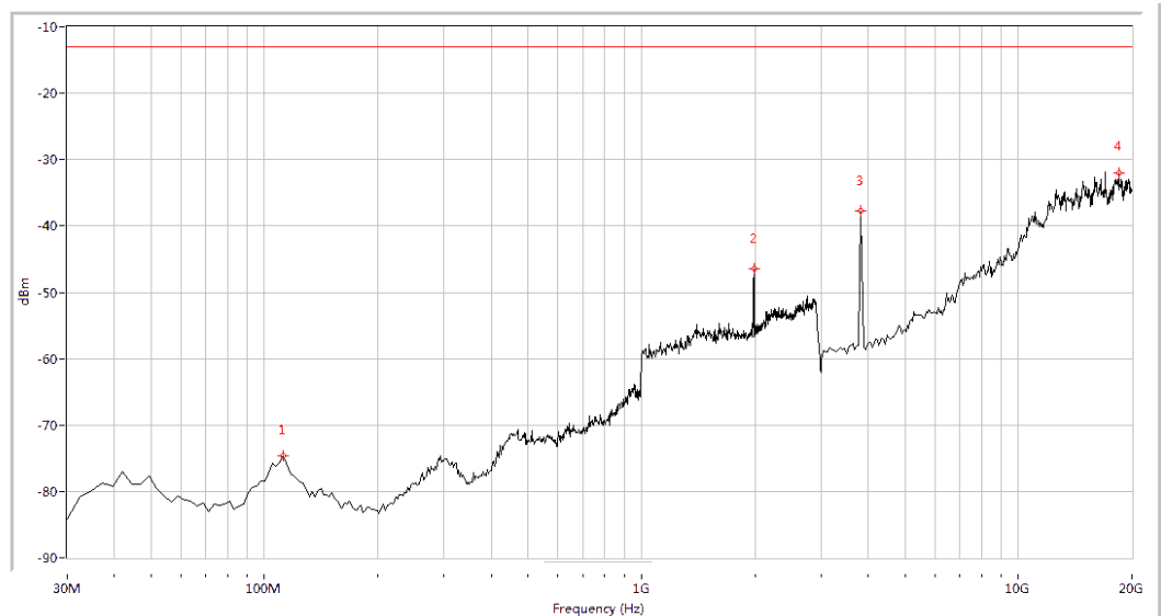
(Plot D.5: WCDMA 1900MHz Channel = 9538, Test Antenna Horizontal)
