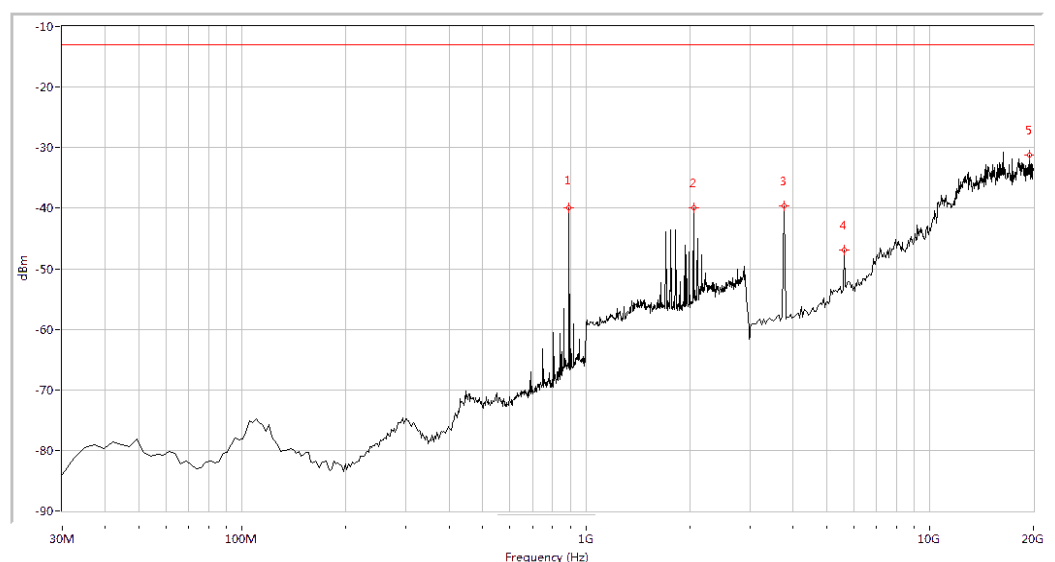
(Plot B.3: GSM 1900MHz Channel = 661, Test Antenna Horizontal)
