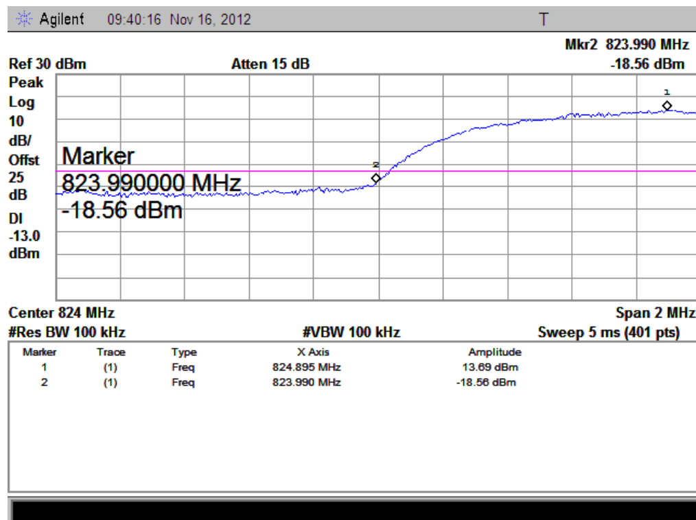
(Plot E: WCDMA 850 Channel = 4132)
