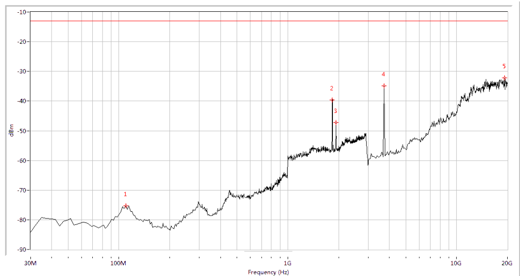
(Plot D.1: WCDMA 1900MHz Channel = 9262, Test Antenna Horizontal)
