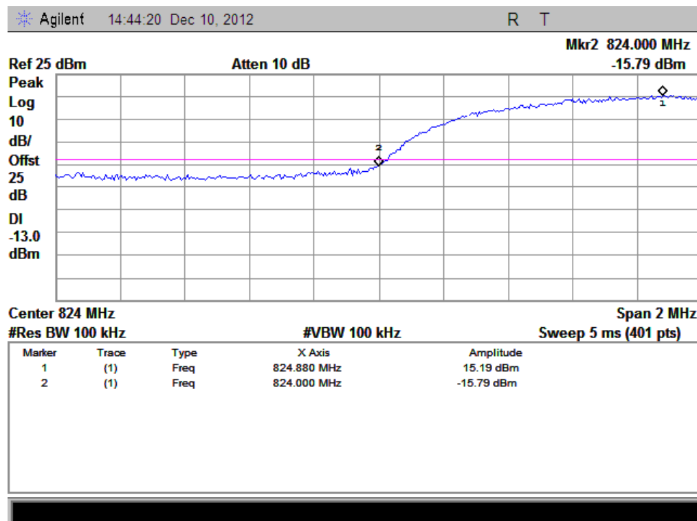
(Plot I: HSDPA 850 Channel = 4132)
