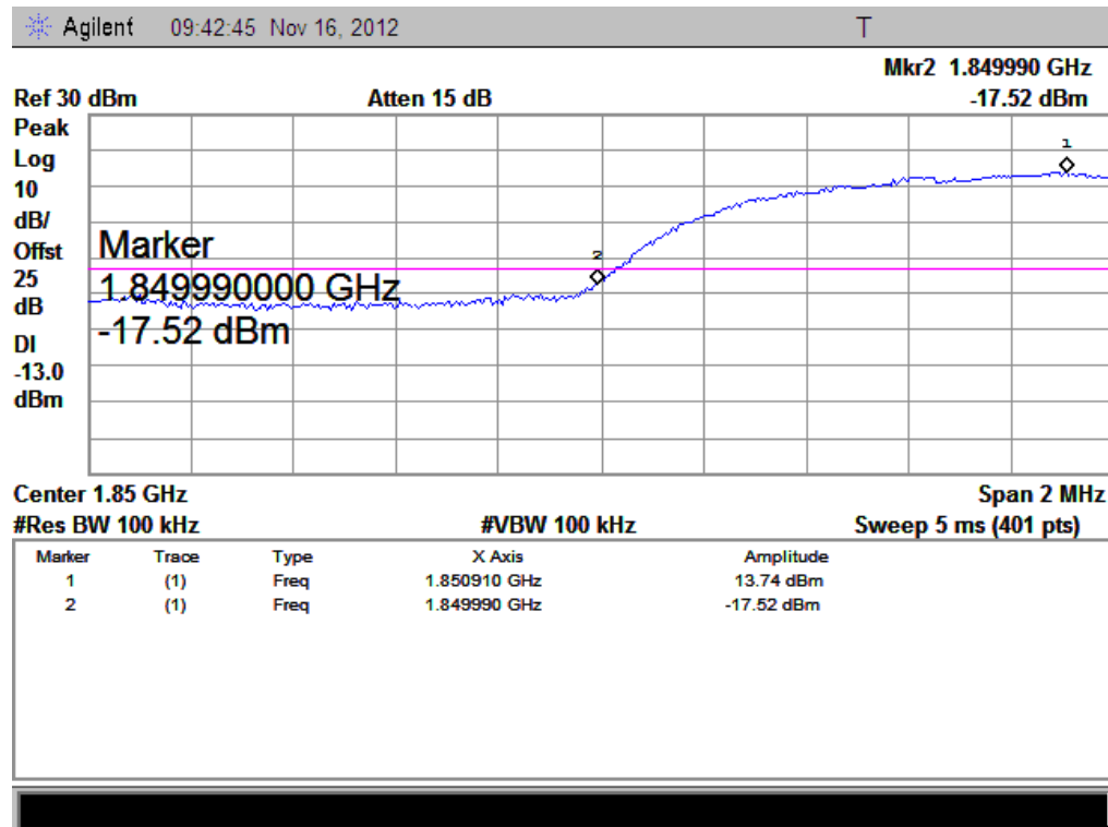
(Plot G: WCDMA 1900 Channel = 9262)
