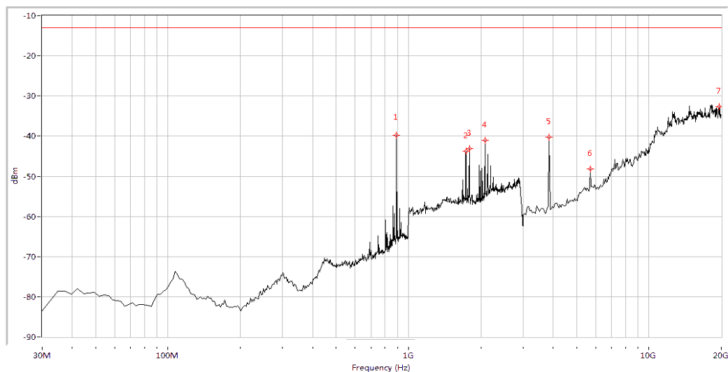
(Plot B.5: GSM 1900MHz Channel = 810, Test Antenna Horizontal)
