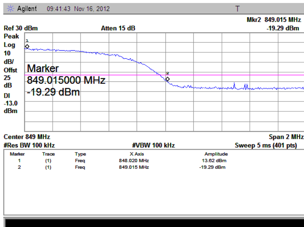
(Plot F: WCDMA 850 Channel = 4233)
