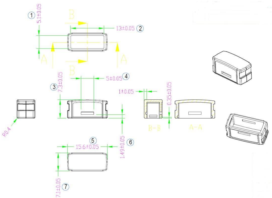
Figure 4. Internal Drawing (Cap)
