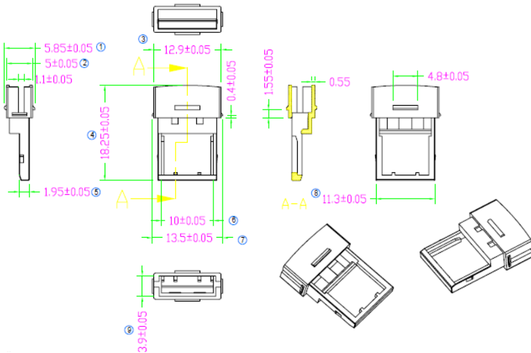
Figure 3. Internal Drawing (Body)
