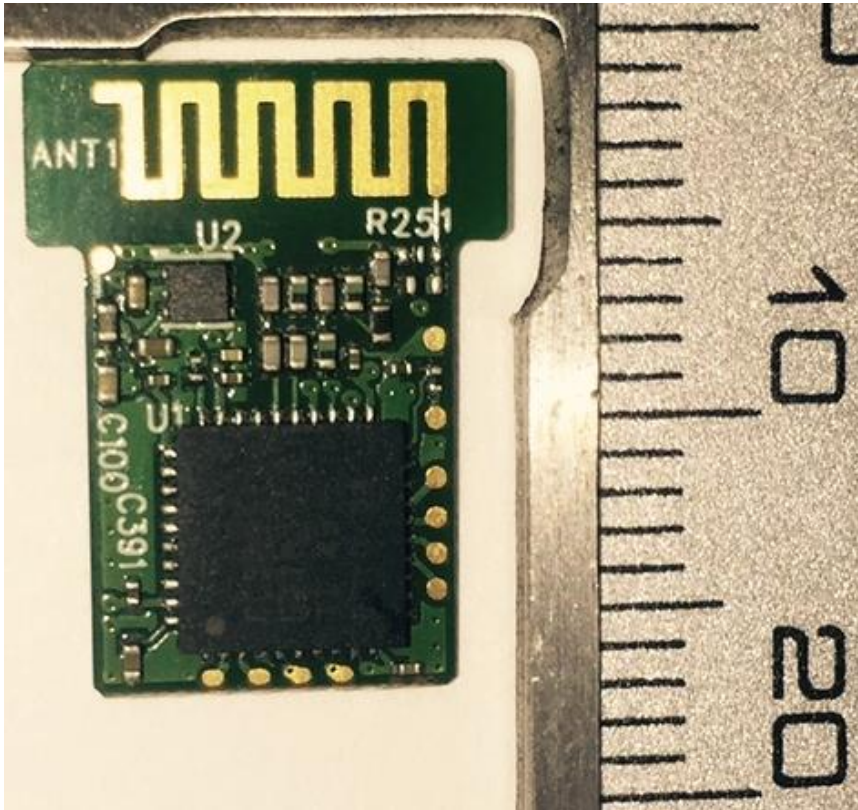
Figure 1. PCBA (Top)
