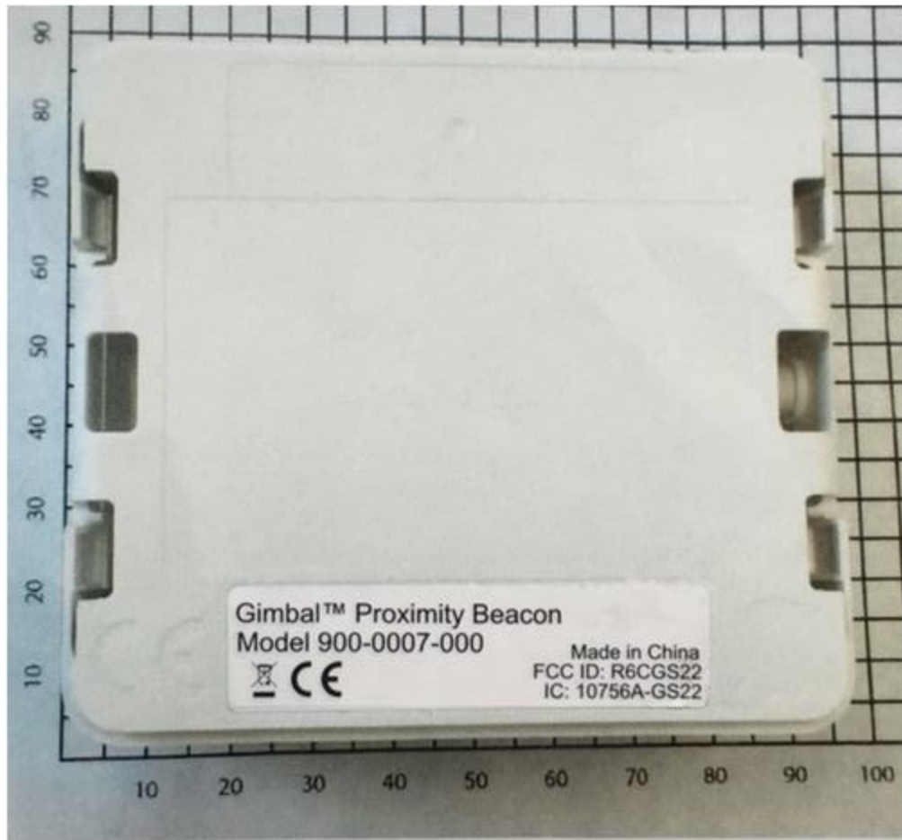
Figure 2: Rear Side
