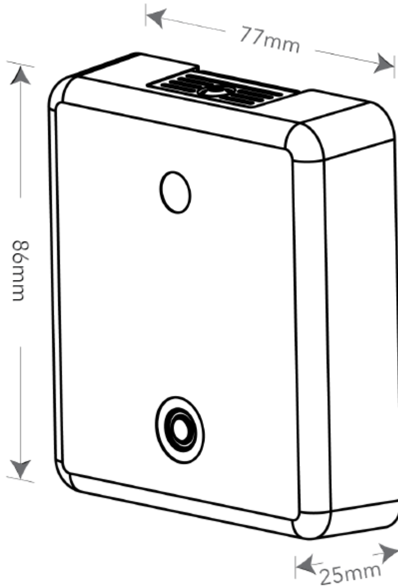
Figure 8: Unit Dimensions
