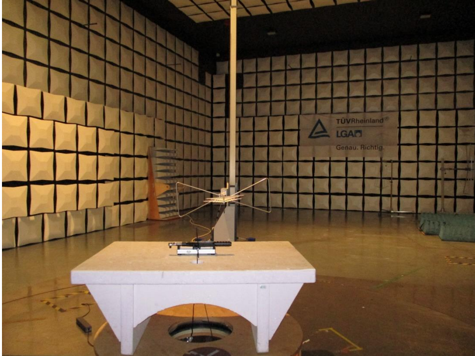
Test Setup: Radiated Measurements (30 MHz - 1 GHz)
