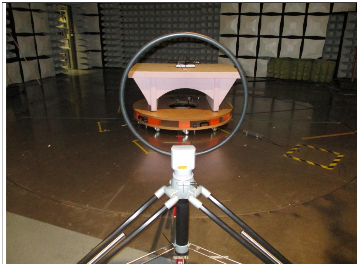
Test setup: Radiated measurements (9KHz -30MHz)
