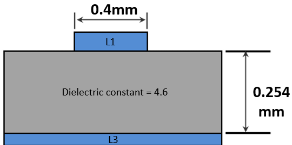
Figure 3: PCB Stack up Guideline
