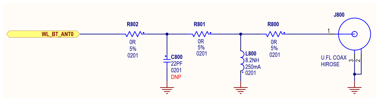
Figure 1: Antenna schematic design guideline
