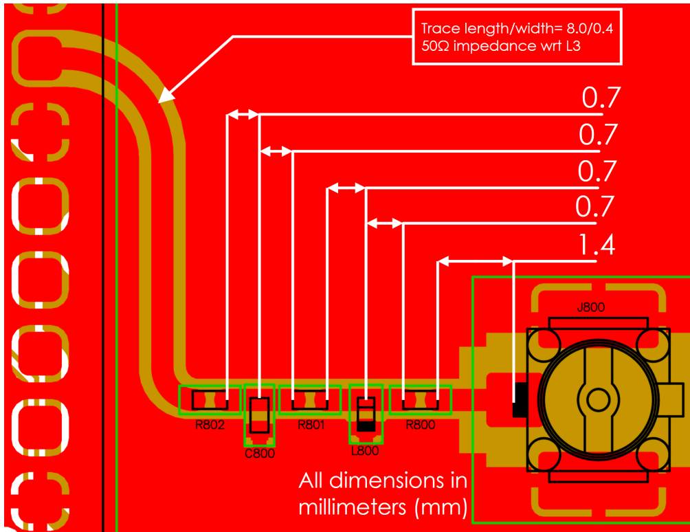
Figure 2. PCB Design Guideline
