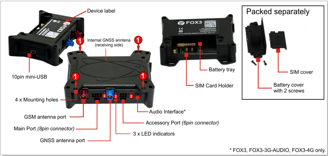
Figure 5: Interface specifications for FOX3-2G/3G/4G devices.
