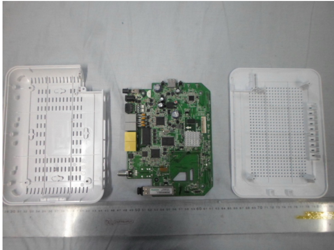
FIGURE 6 GPON SFU (M/N: 7262G) COVER REMOVED
