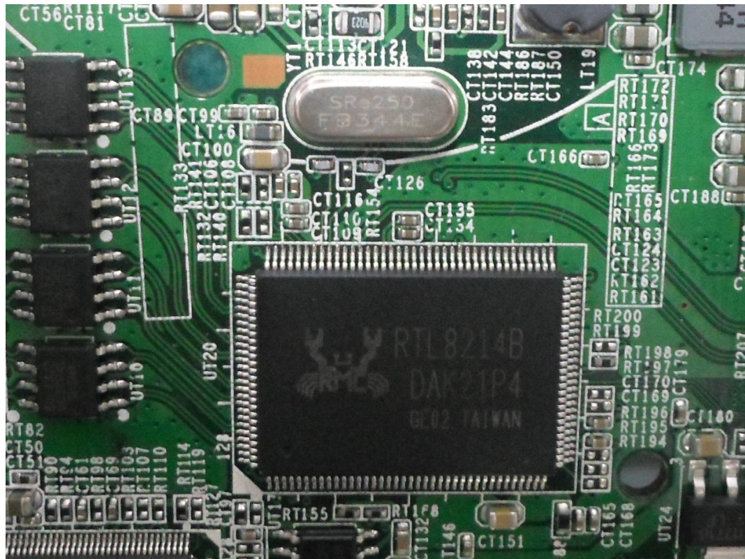
FIGURE 9 GPON SFU (M/N: 7262G) CHIP AND CRYSTAL ON MAIN BOARD
