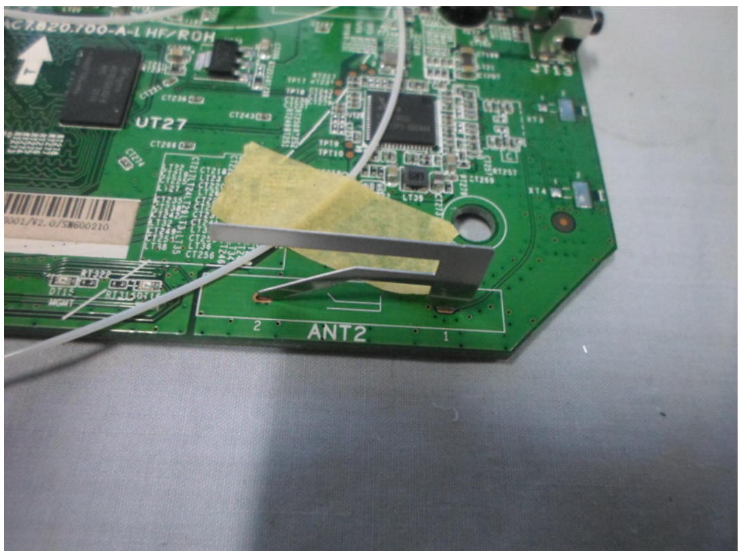
FIGURE 12 GPON SFU (M/N: 7262G) ANT2
