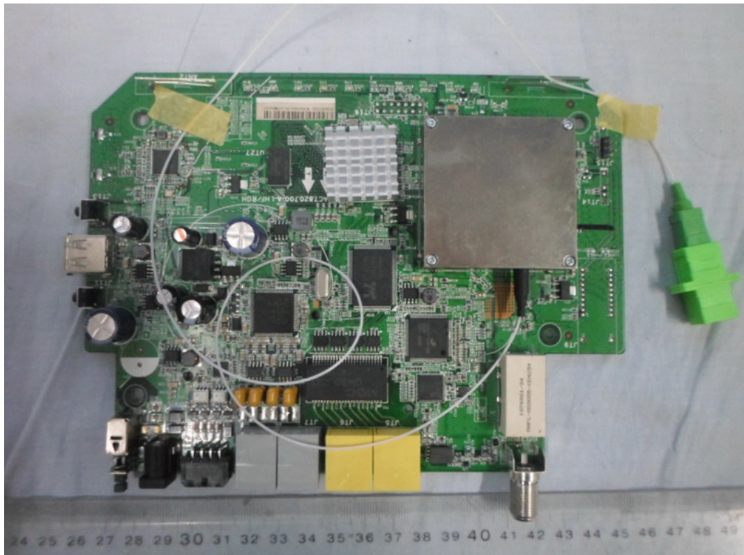
FIGURE 7 GPON SFU (M/N: 7269G) MAIN BOARD (COMPONENT SIDE)
