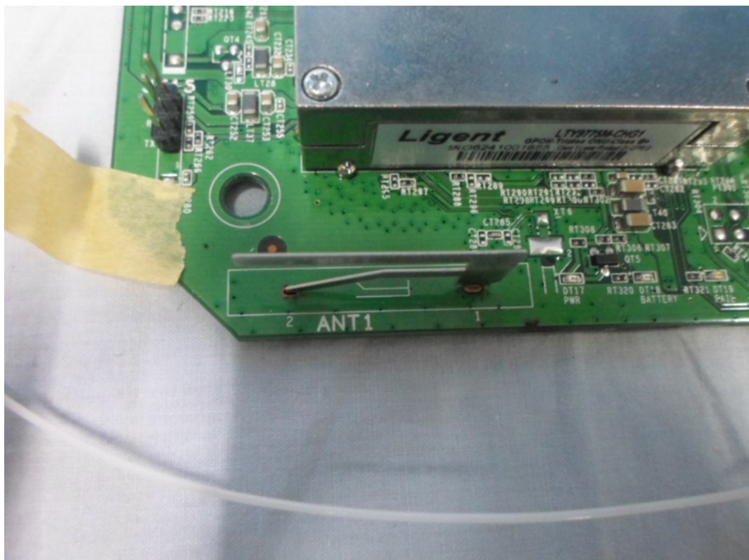
FIGURE 12 GPON SFU (M/N: 7269G) ANTI
