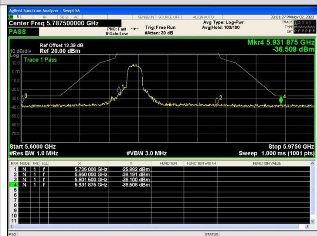
Out Of Band Emission IEEE 802.11n_Channel 149_20MHz_Antenna 0
