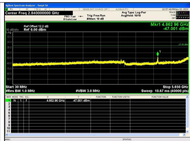
Spurious Emission:30.0~5650 MHz IEEE 802.11a_Channel 165_20MHz_Antenna 0
