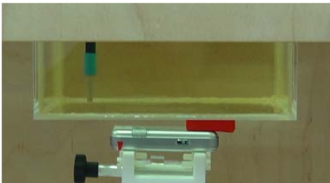
Fig.10 Side Position (The distance between the back of the device and the bottom of the flat phantom is 1.5cm.)
