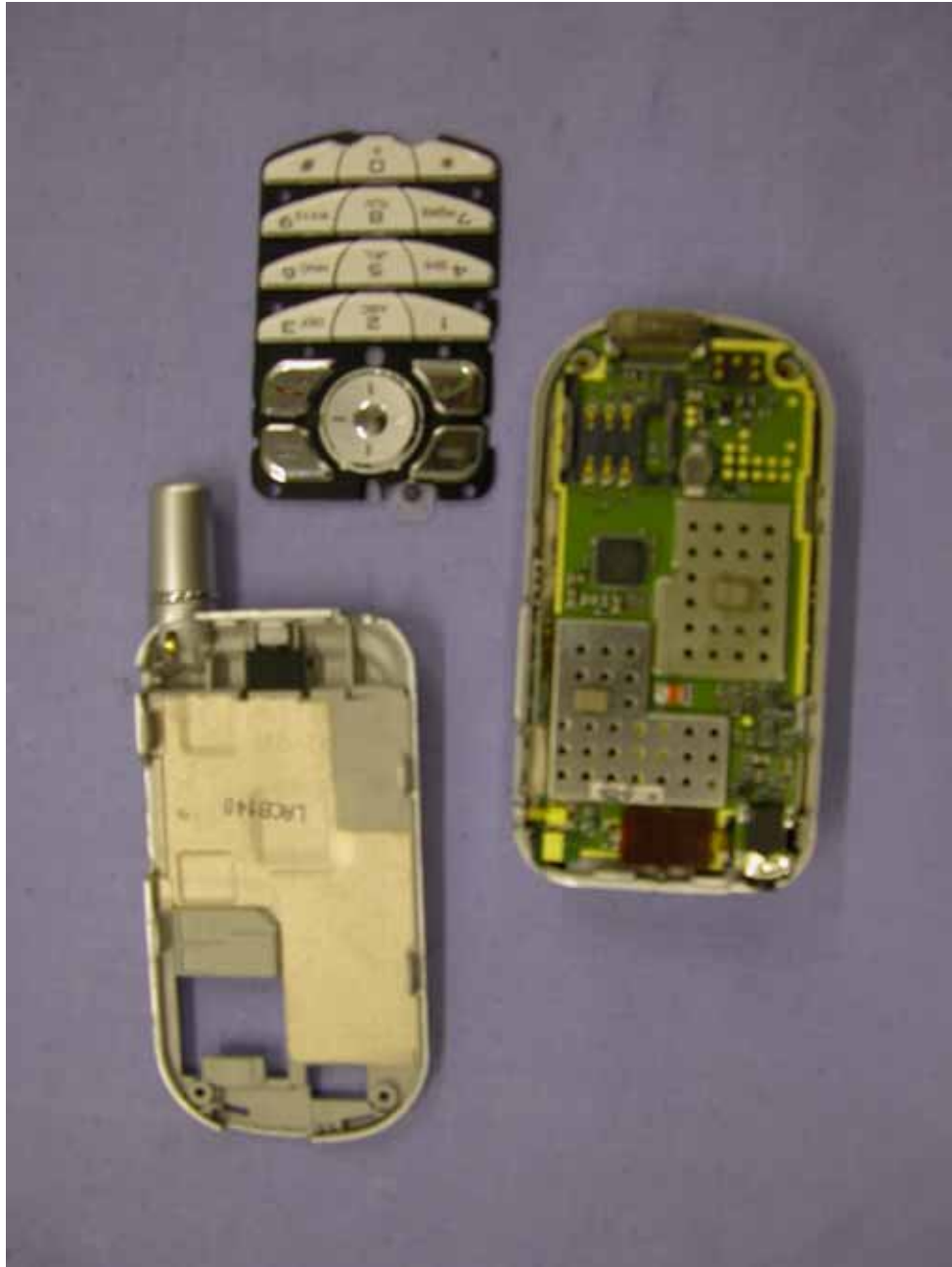
Mobile phone Disassembly
