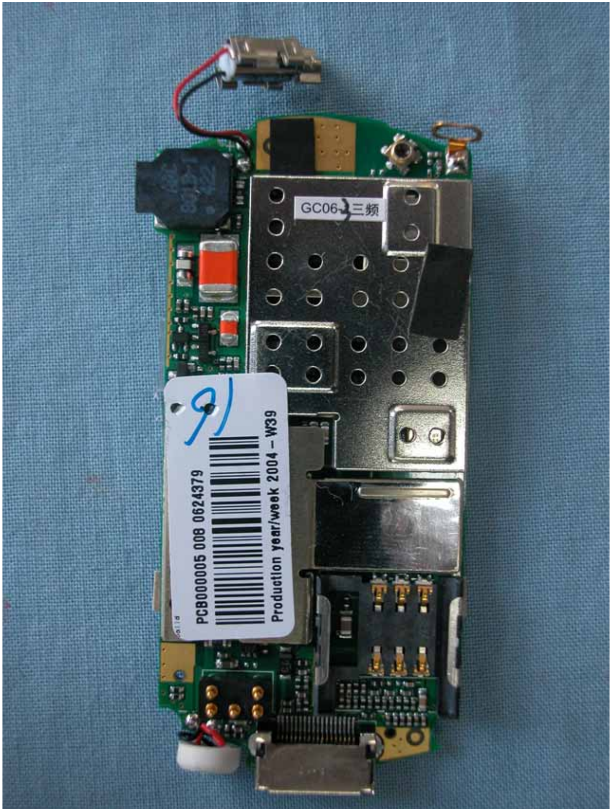
TCL538 PCB rear view
