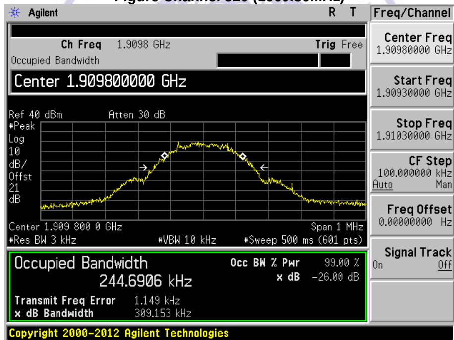
Figure Channel 810 (1909.80MHz)
