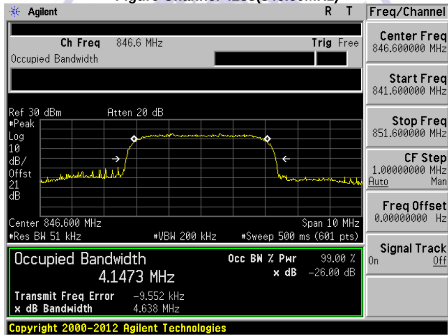
Figure Channel 4233(846.60MHz)
