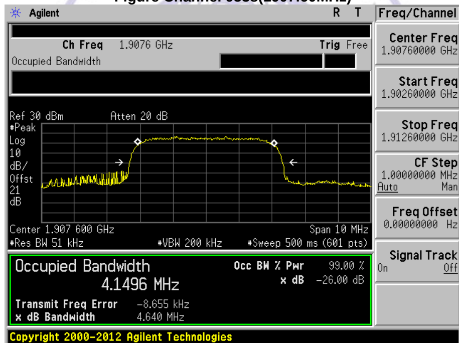
Figure Channel 9538(1907.60MHz)
