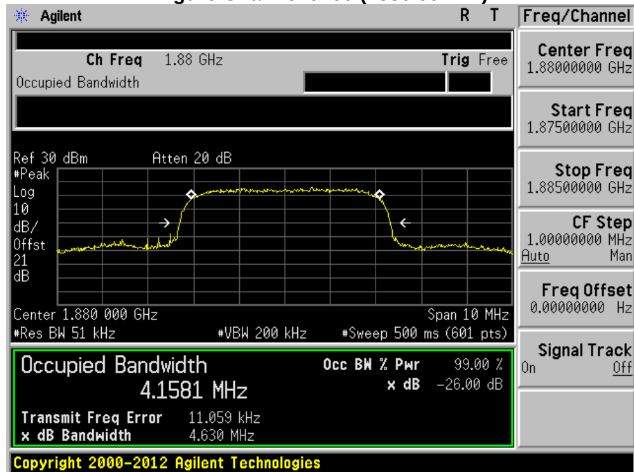
Figure Channel 9400 (1880.00MHz)
