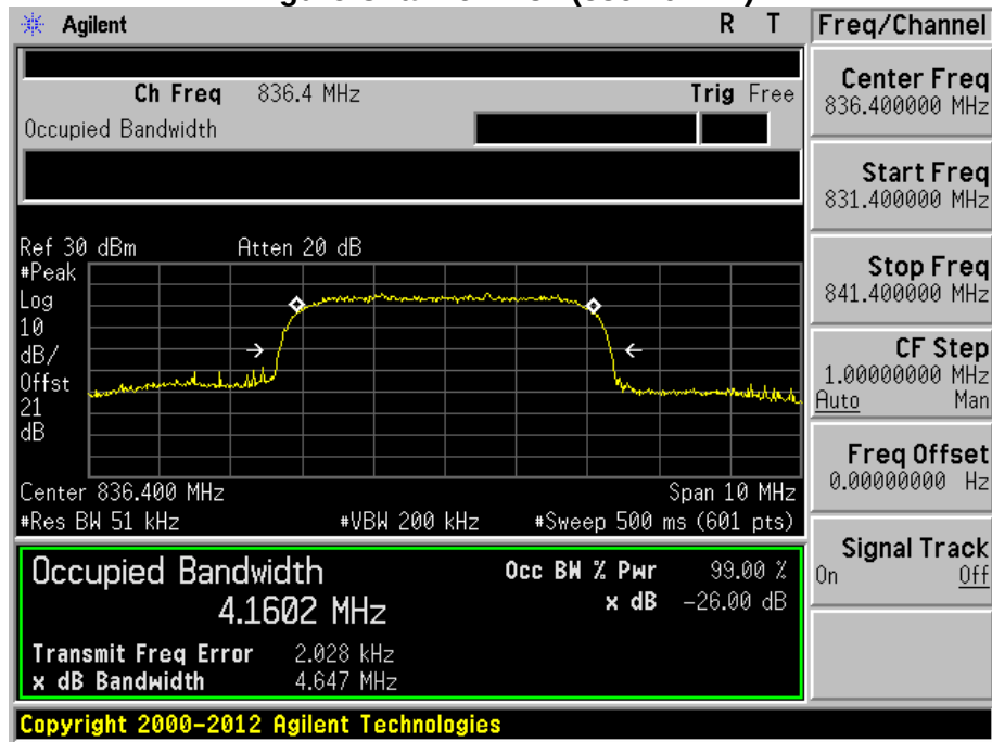
Figure Channel 4182 (836.40MHz)
