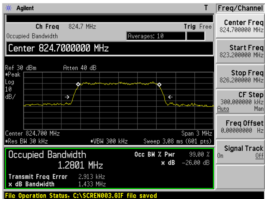
CDMA Cellular CH1013 Occupied Bandwidth
