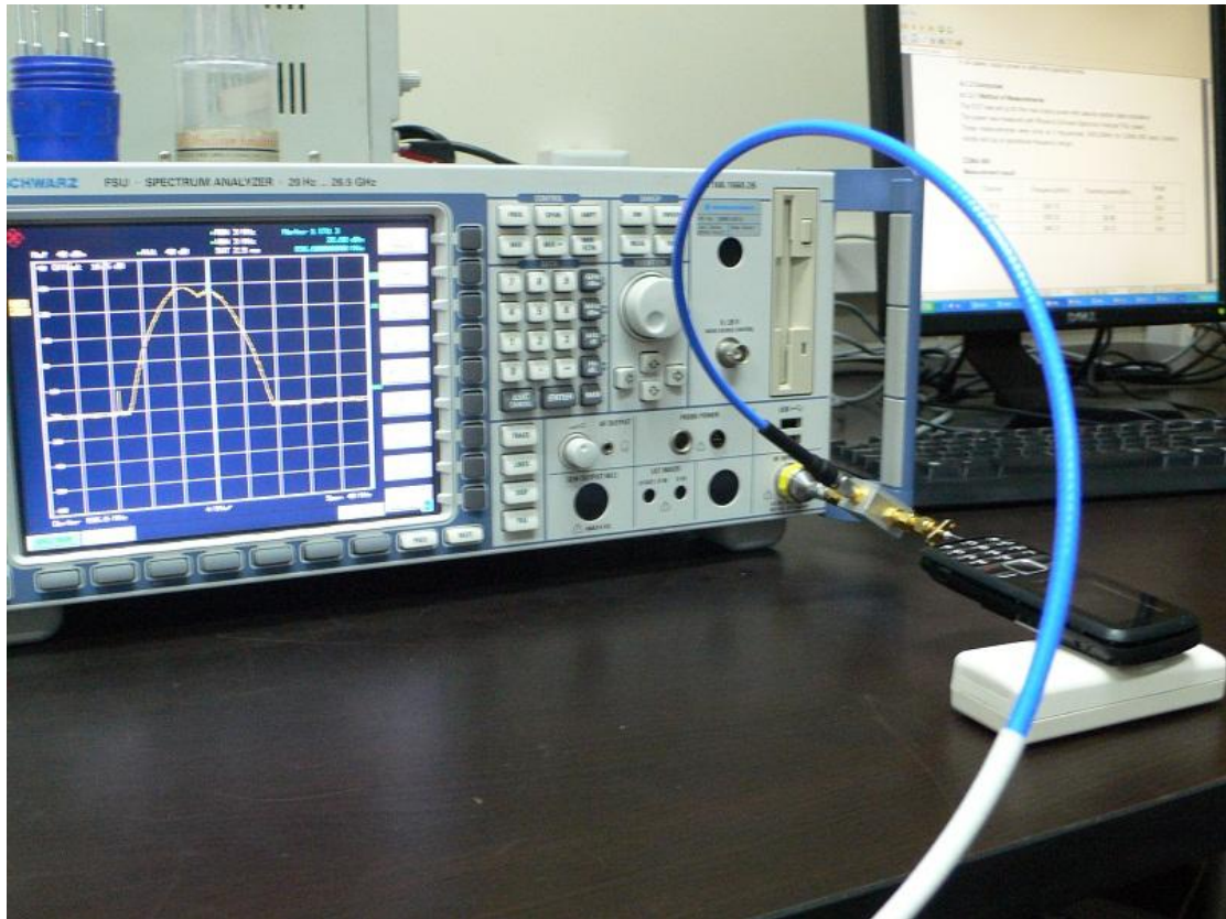
RF test
