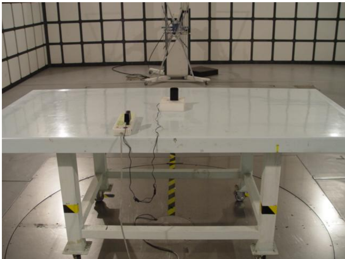
RSE test
