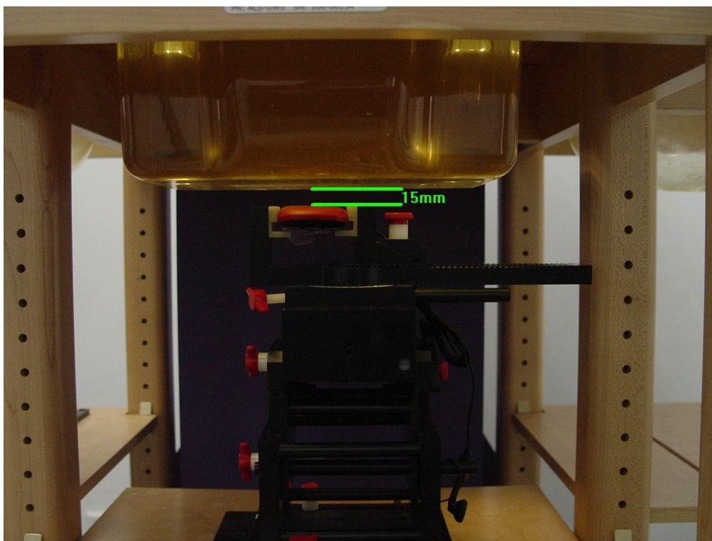
Figure B.6 EUT Body Towards Ground with earphone
