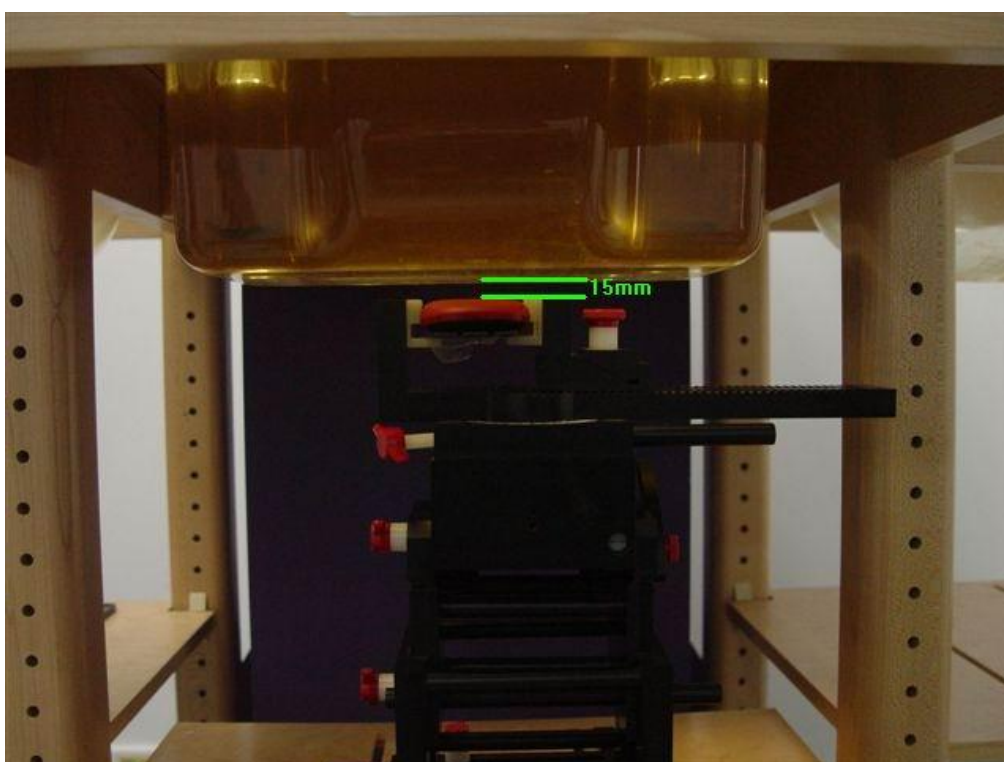
Figure B.6 EUT Body Towards Ground
