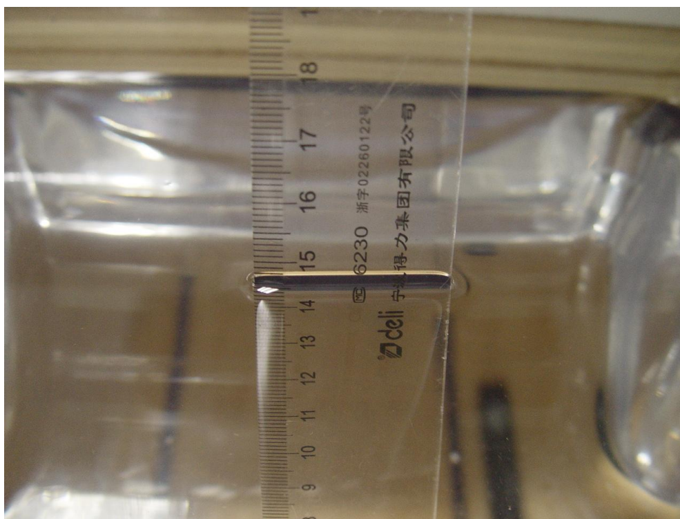
Figure B.1 Depth of Simulating Liquid in SAM Head Phantom
