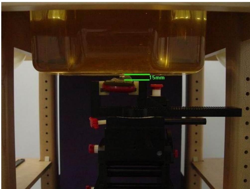
Figure B.6 EUT Body Towards Phantom
