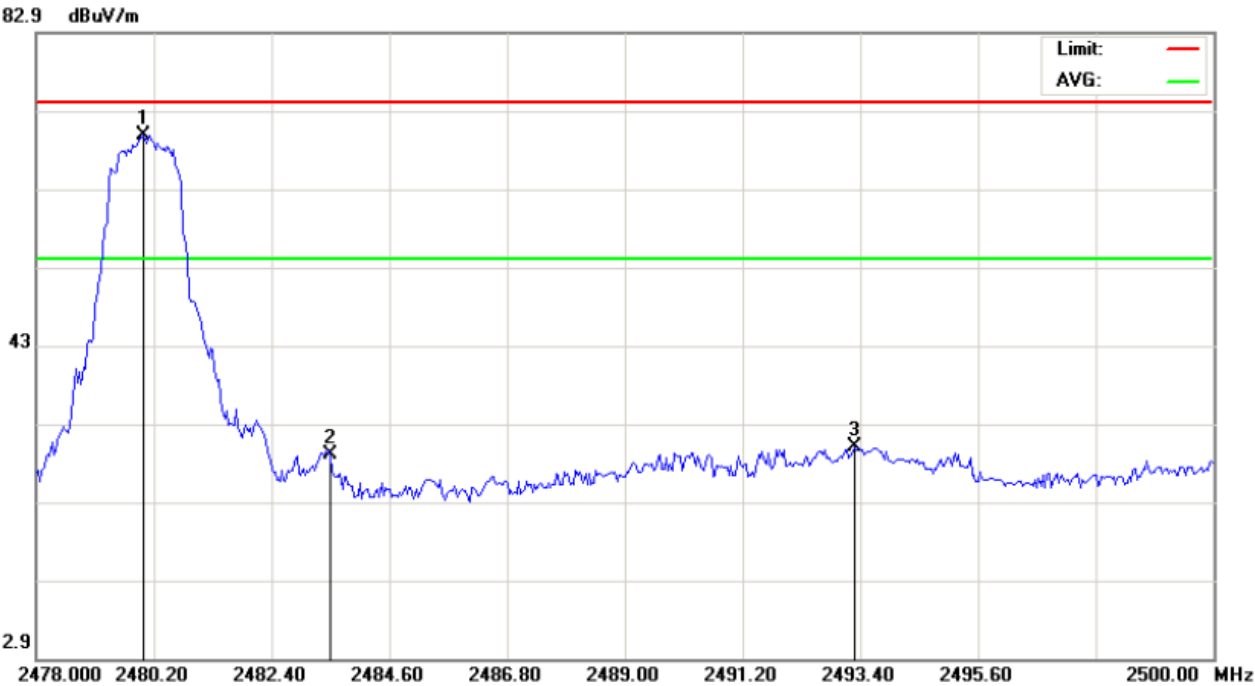
TEST PLOT OF BAND EDGE FOR HIGH CHANNEL (3Mbps)-Vertical
