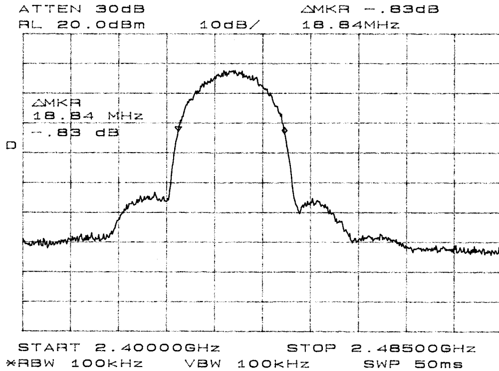
Figure 9 Band width plot taken in screen room.
