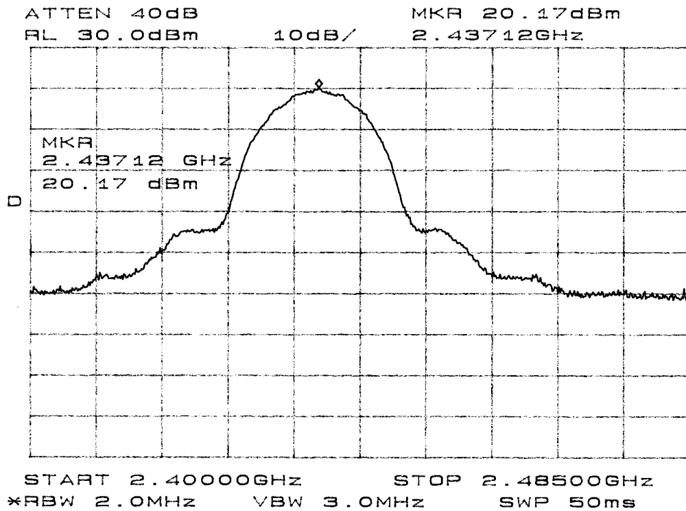
Figure 10 maximum output power plot taken in screen room.
