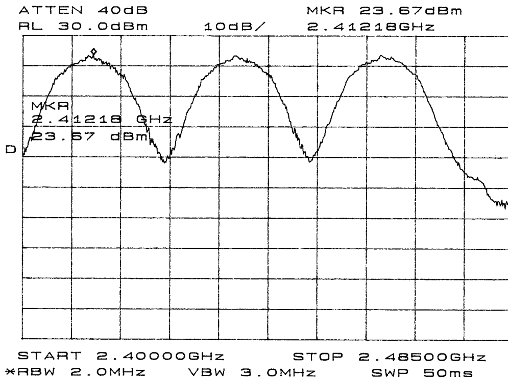
Figure 8 band edge and maximum power plot taken in screen room.
