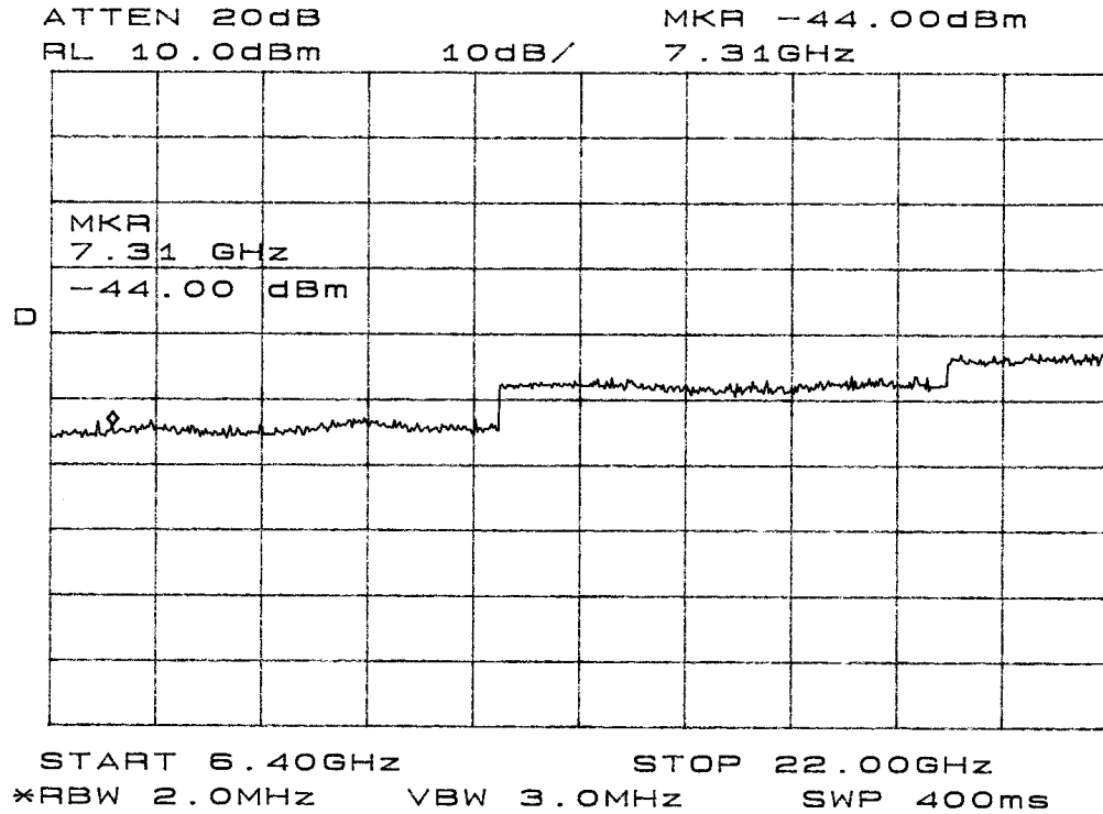
Figure 13 Antenna Emission plot taken in screen room.
