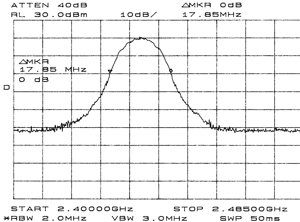
Figure 9 Band width Requirement plot taken in screen room (mode B).
