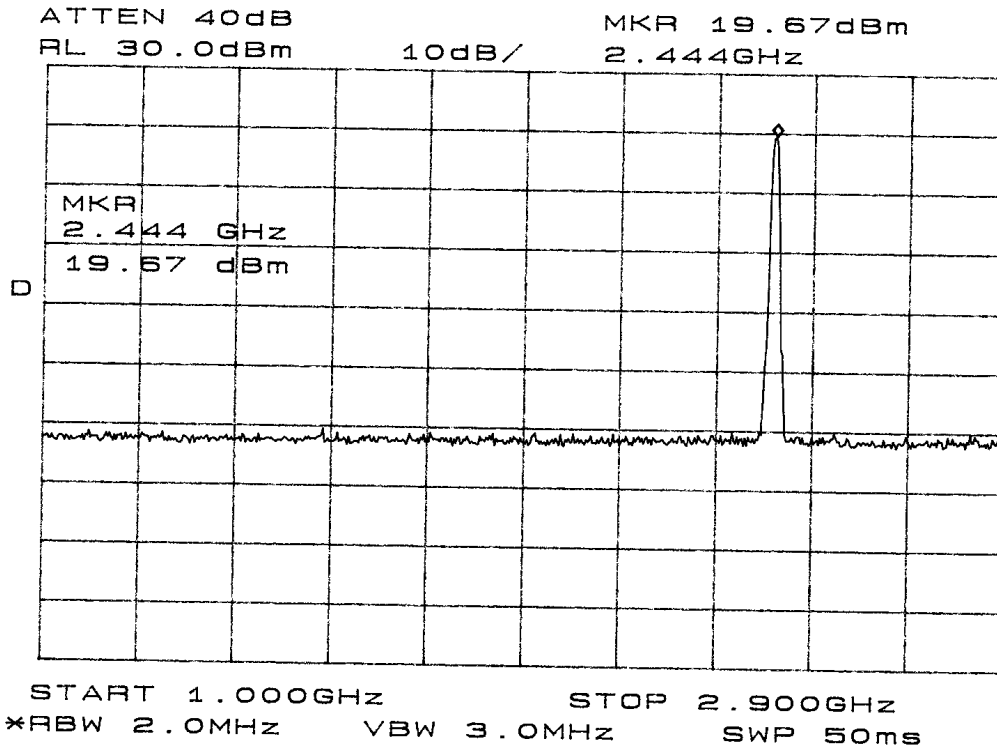
Figure 11 Antenna Emission plot taken in screen room.
