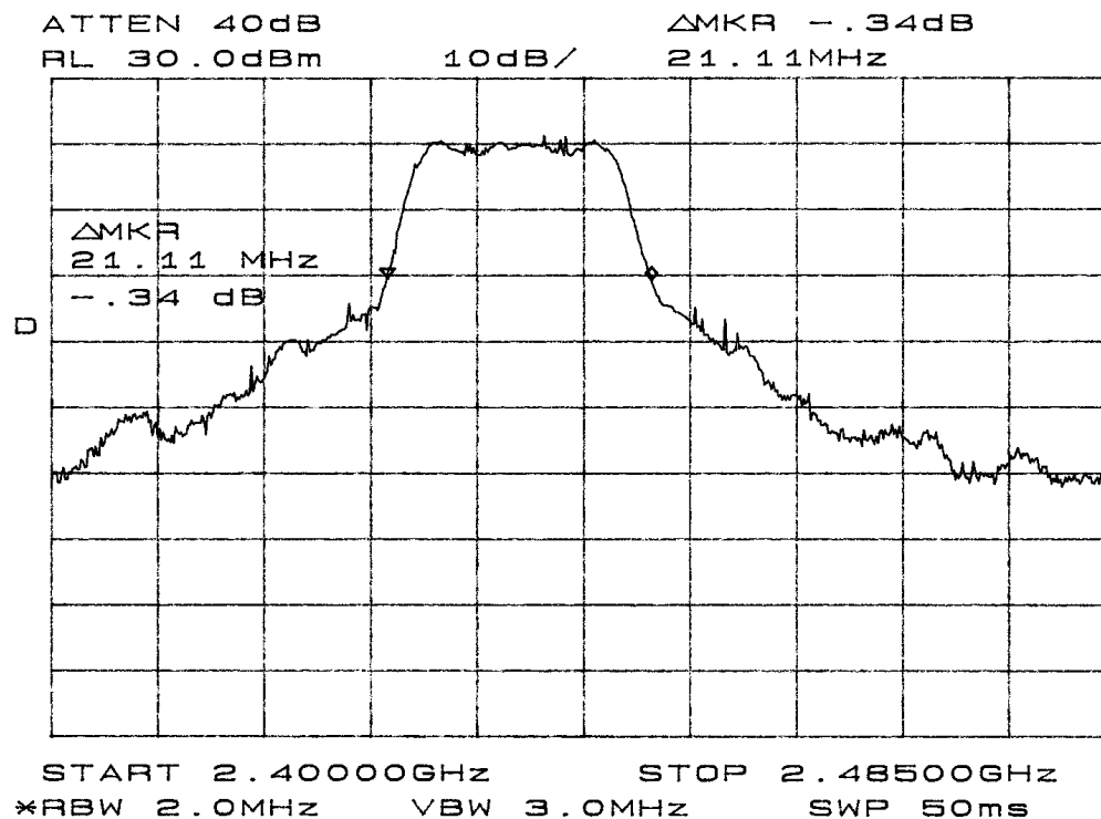
Figure 10 Band width Requirement plot taken in screen room (Mode G).
