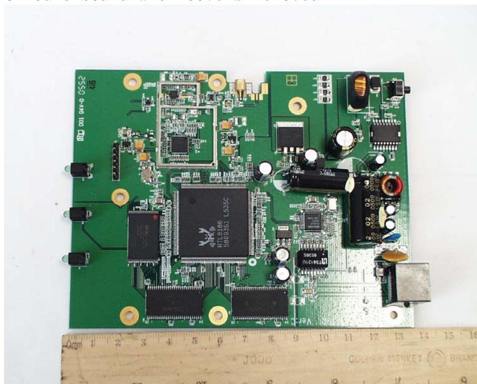
Circuit board with covers removed
