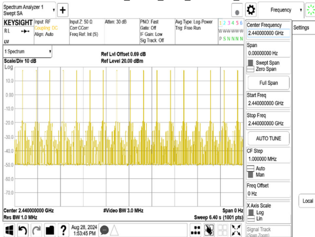
Dwell Time_QPSK_SRD_2440MHz_2
