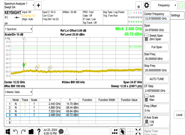
Spurious Emission_QPSK_SRD_2440MHz
