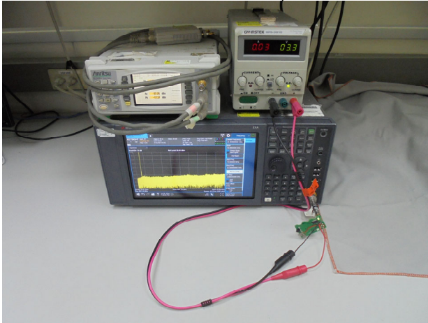
SRD_Radiated_966 (1)_Setup
