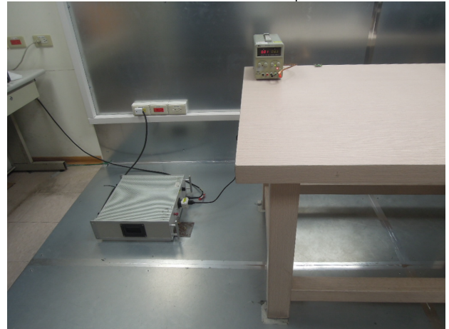
SRD_Conduction_Setup
