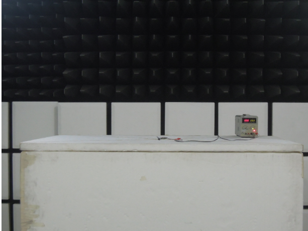
SRD_Radiated_966 (2)_Setup
