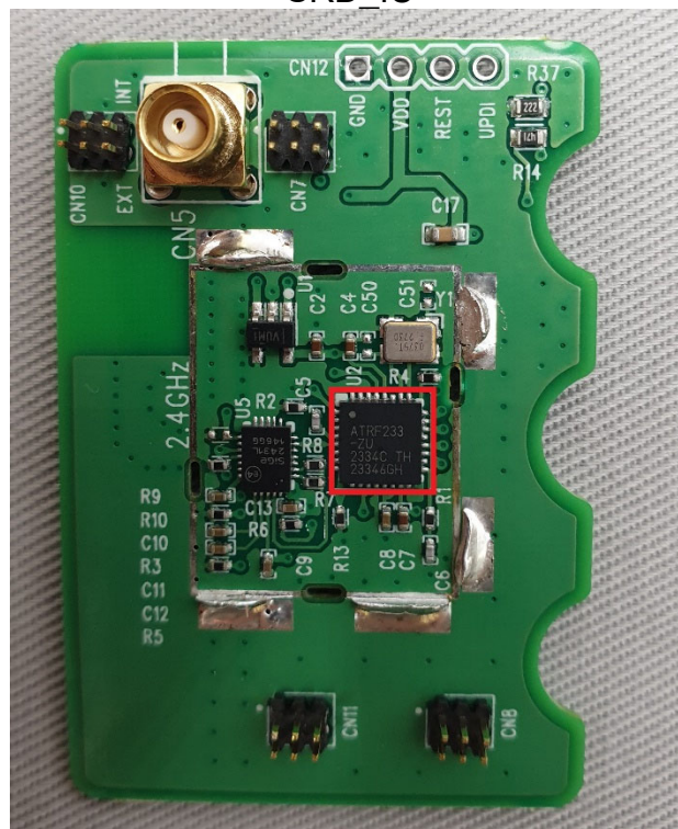
SRD_IC
