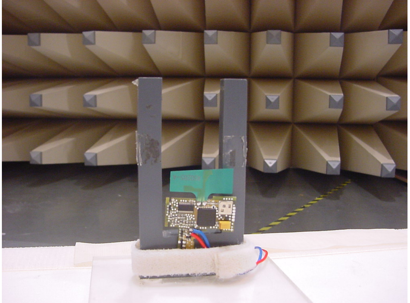
Photo 2: Radiated Emissions
