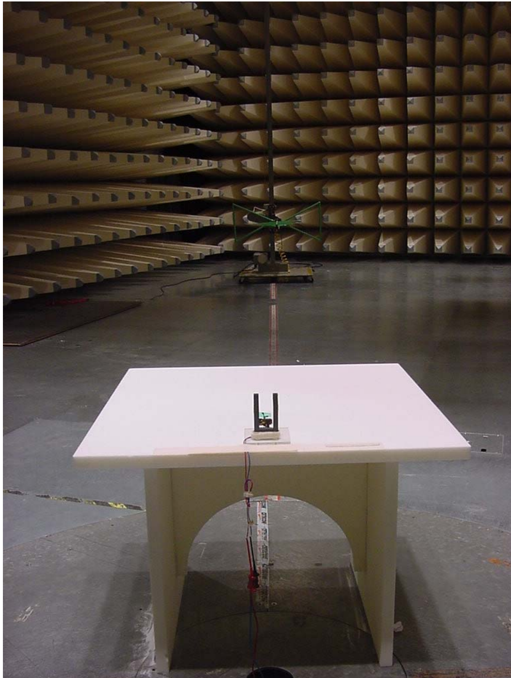
Photo 1: Radiated Emissions
