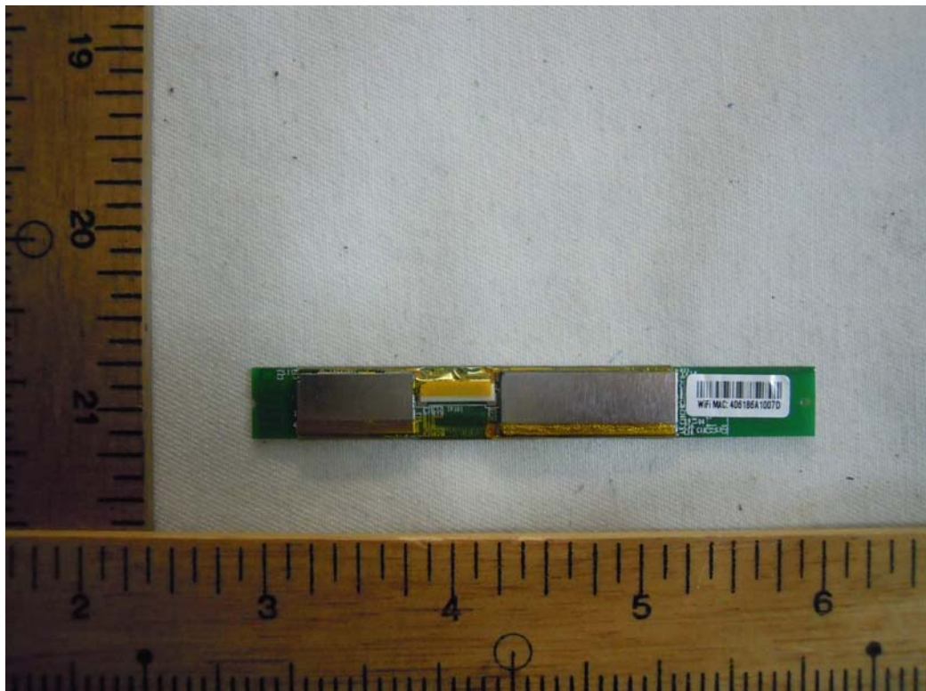
18. Front view of PCB4
