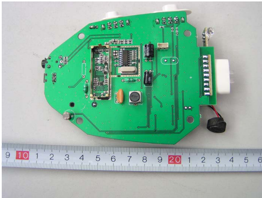
EUT - PCB 1 Unshielded Bottom View
