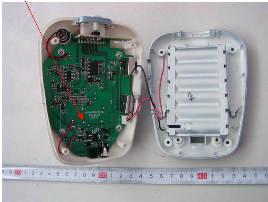
EUT – EUT Inside View
