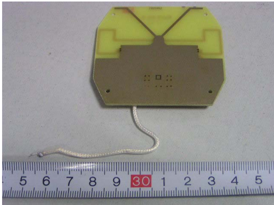
EUT- Antenna PCB Back View
