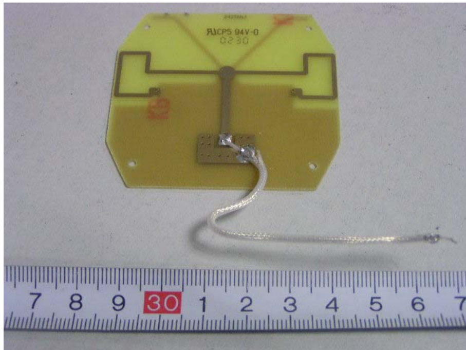
EUT- Antenna PCB Front View
