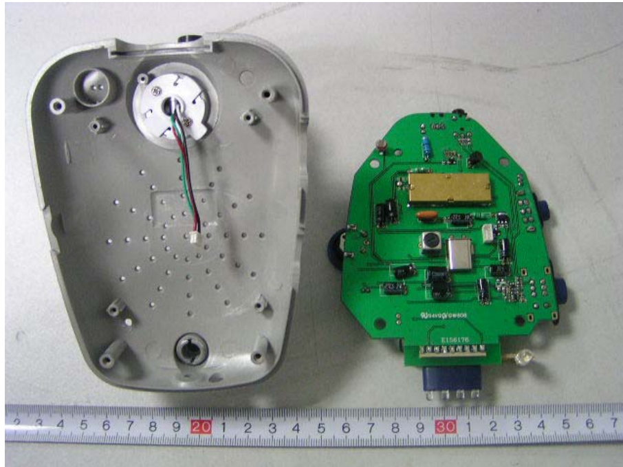
EUT-Inside View (3)
