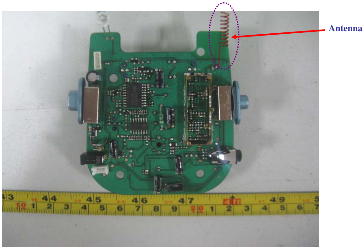
EUT – Control Board Bottom Components View
