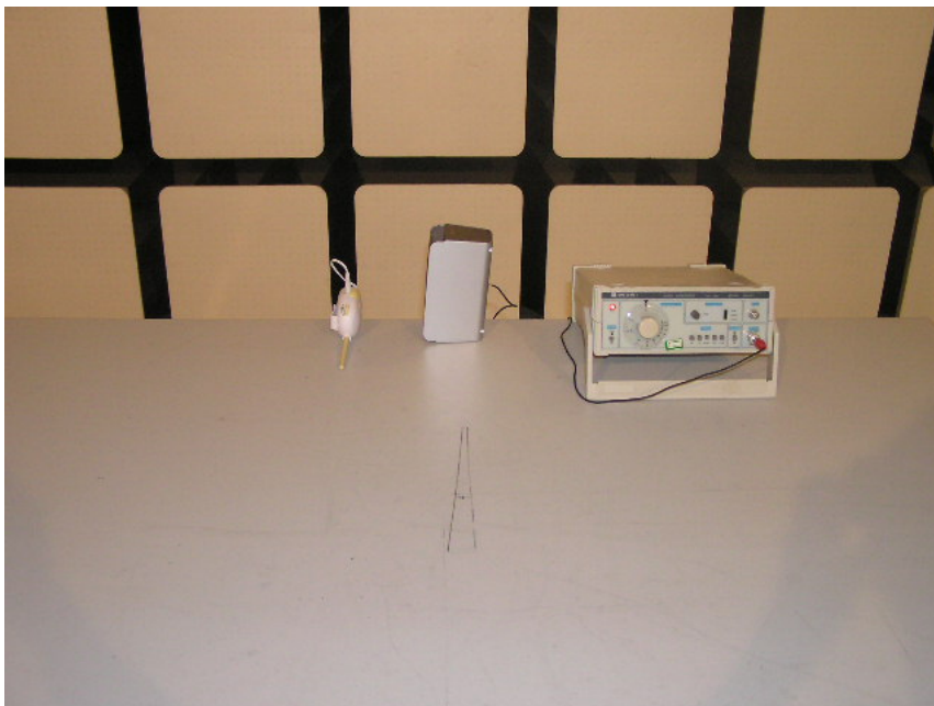
Radiated Emissions-Side View
