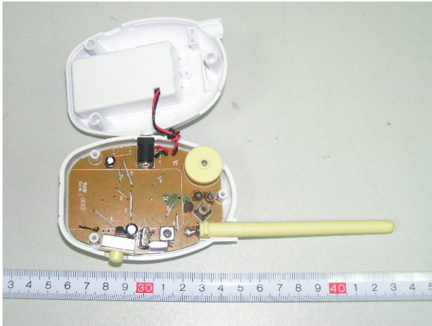
EUT-Uncovered View
