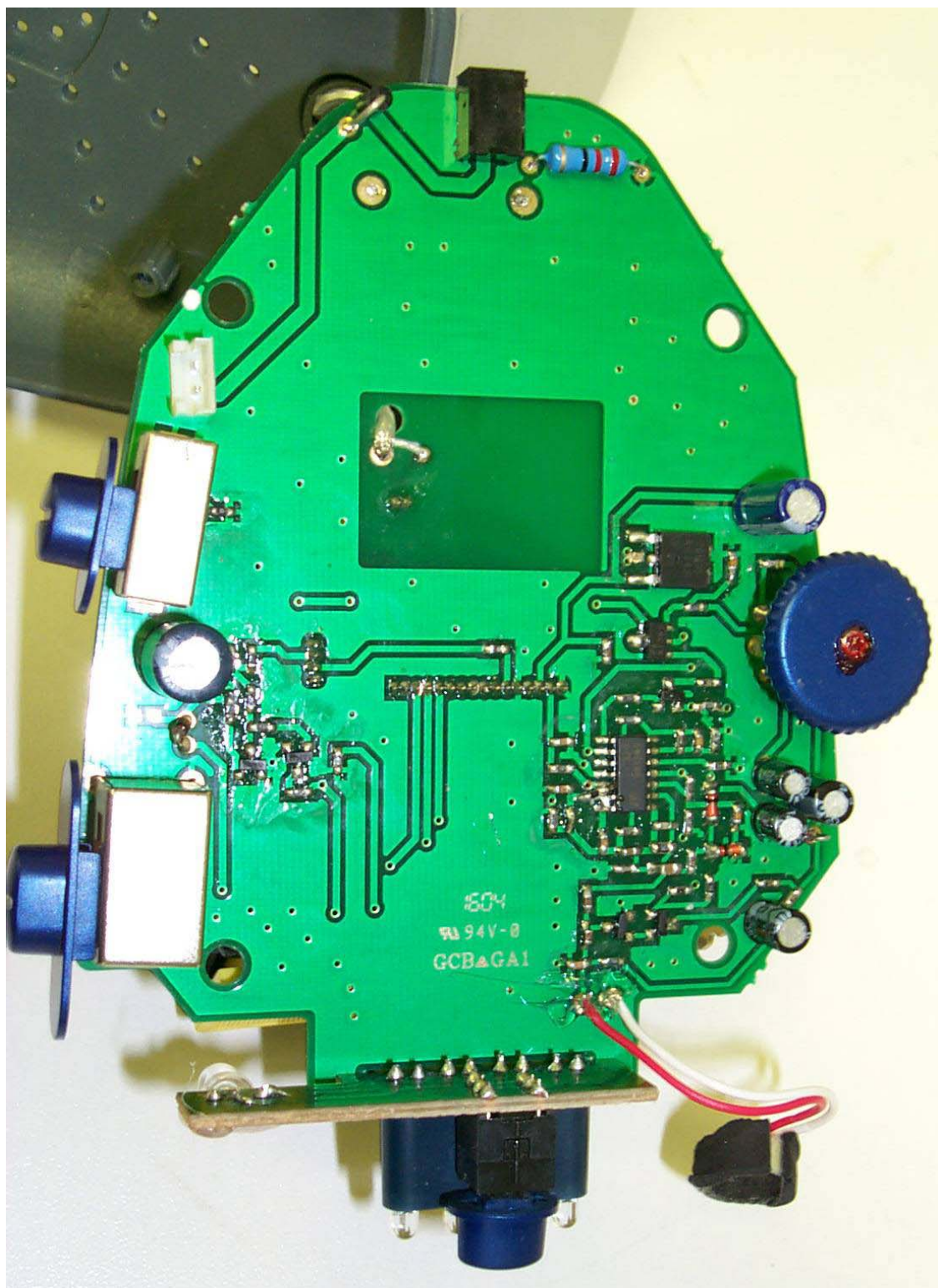
Figure 7.4 PCB Component Side
