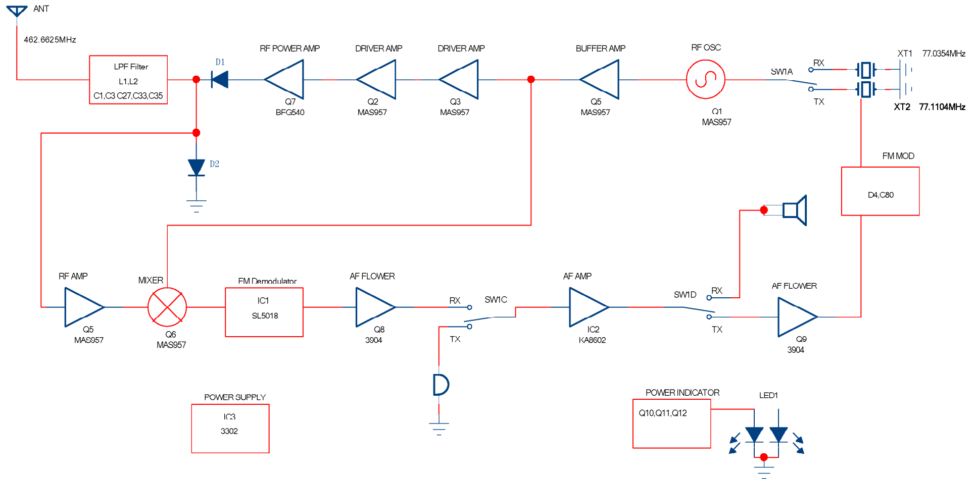
5M5 FRS Walkie Talkie Block Diagram
