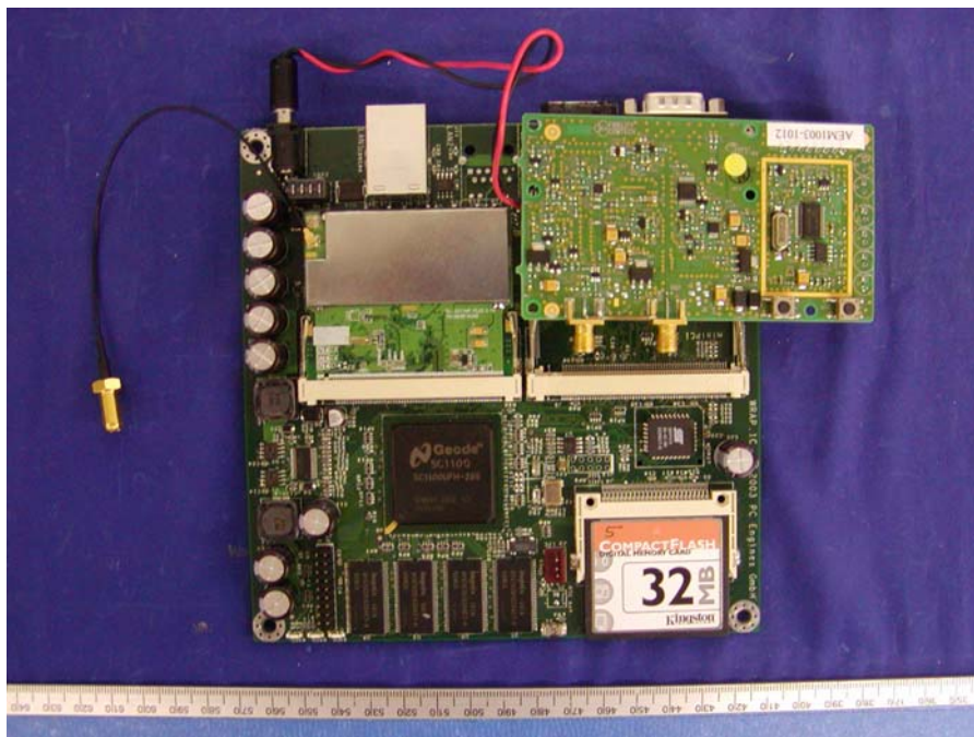
EUT – Main Board Component with Transceiver View
