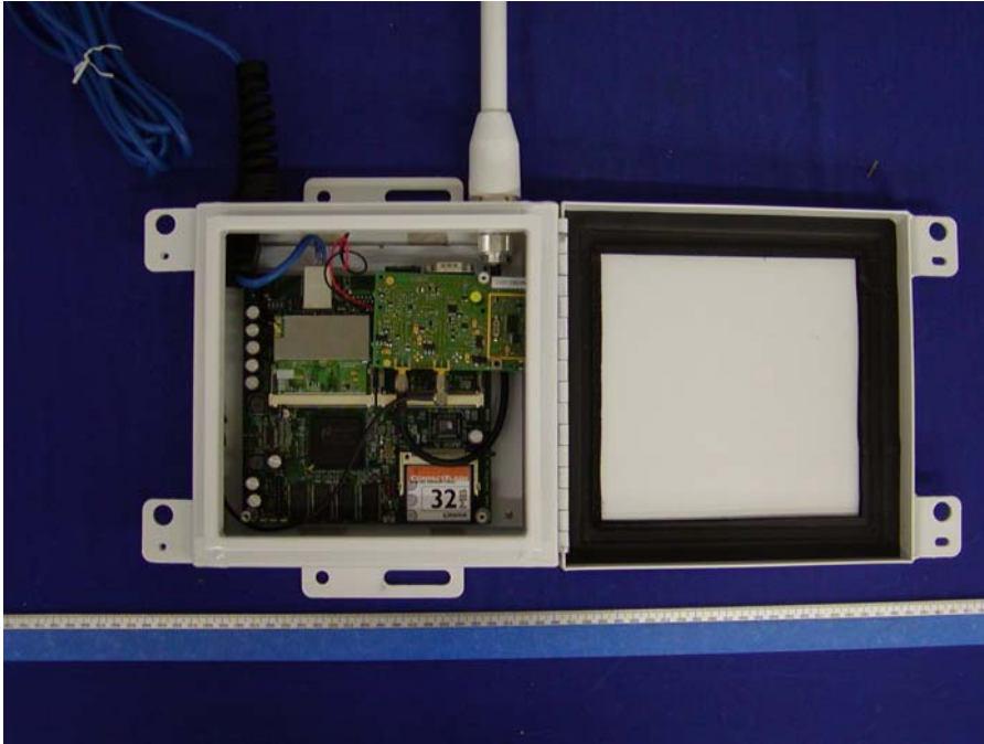
EUT – Chassis Cover Off View
