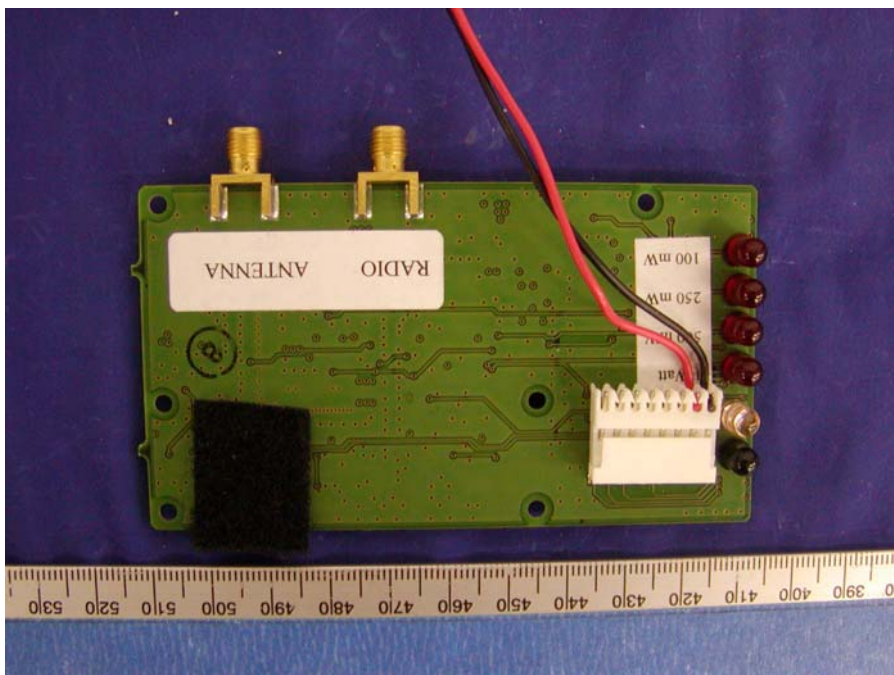
EUT – RF Interface Board Solder View
