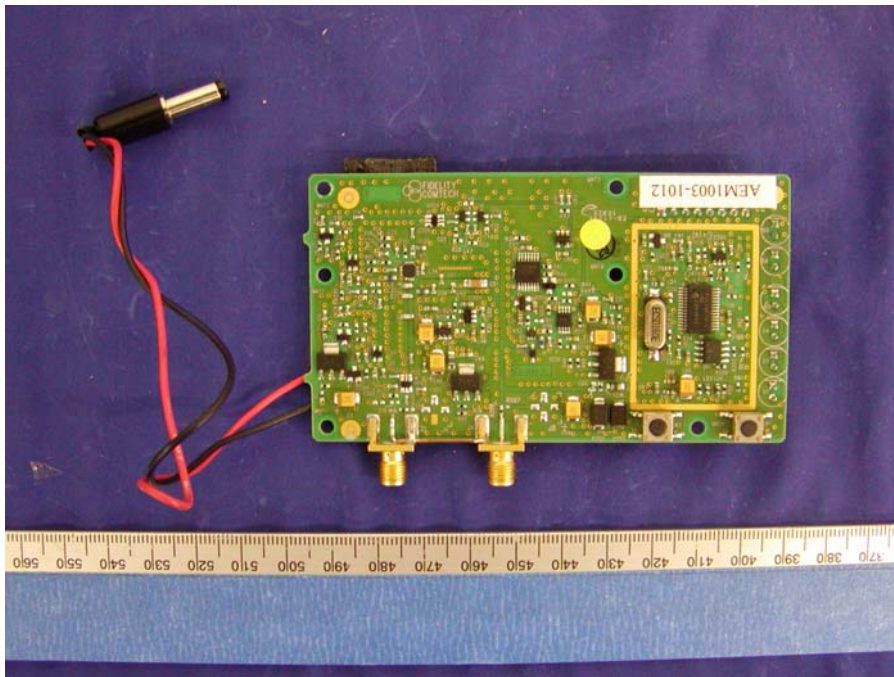
EUT – RF Interface Board Component View
