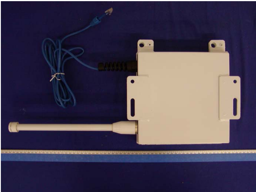
EUT – Chassis Bottom View
