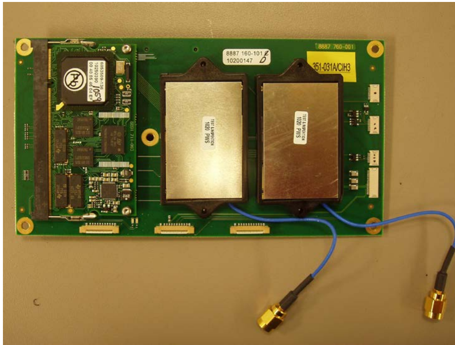
Radio PCB Topside (Shields Installed)
