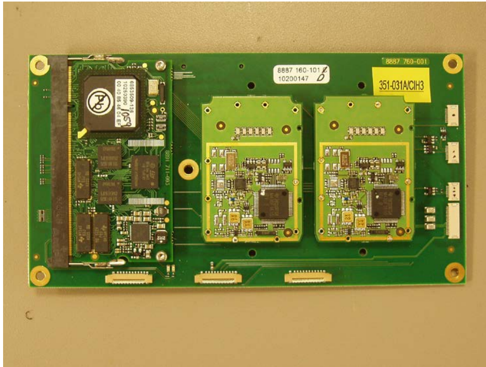
Radio PCB Topside (Shields Removed)
