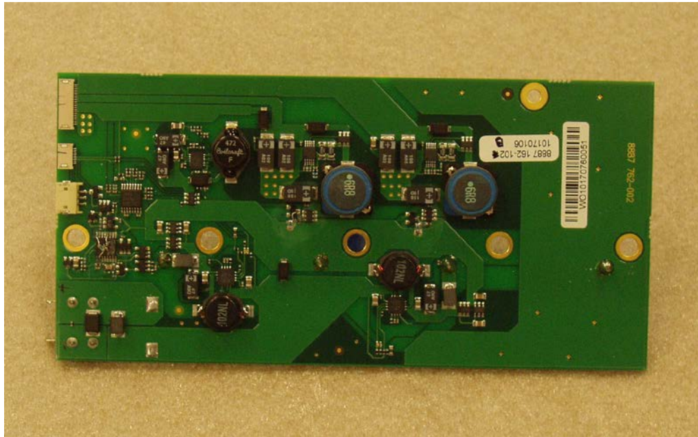
Power Supply PCB Topside
