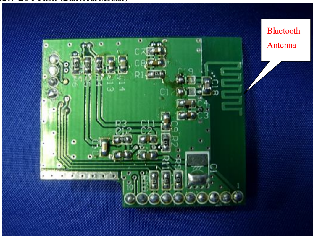
(20) EUT Photo (Bluetooth Module)
