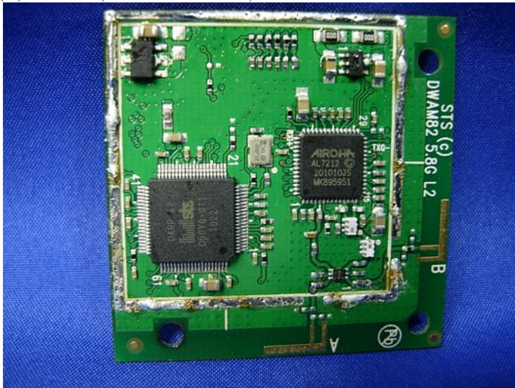
(24) EUT Photo (5.8GHz Transmit Module)
