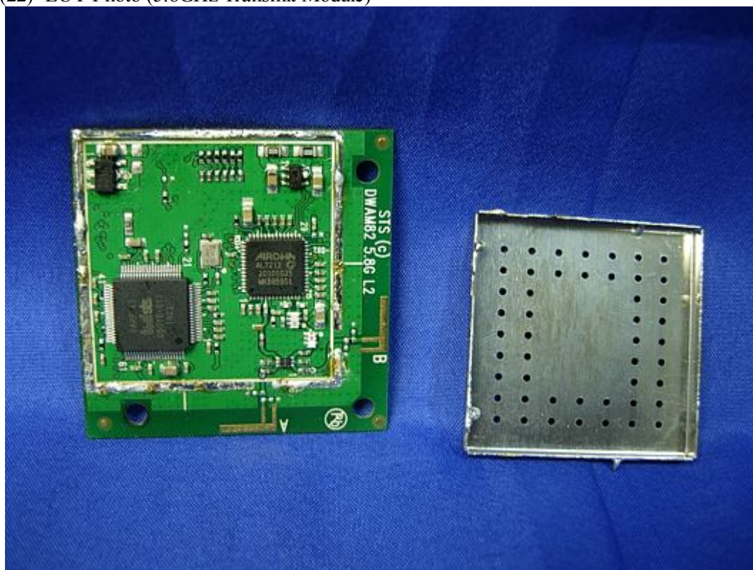
(22) EUT Photo (5.8GHz Transmit Module)
