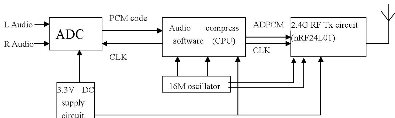
EB35E0TP Block Diagram
