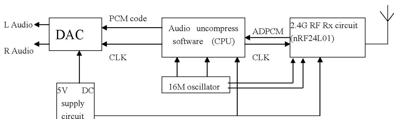
EB35E0RP Block Diagram
