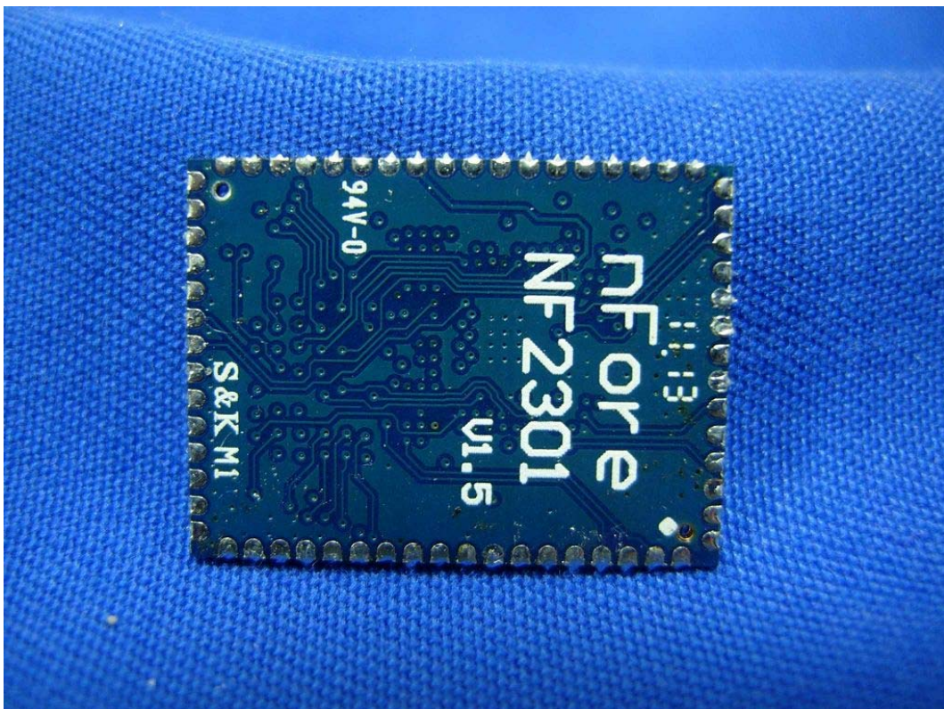
(26) EUT Photo-(BT)
