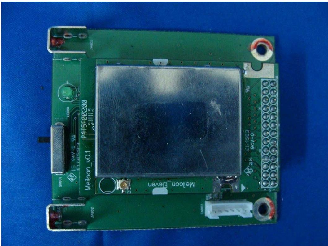
(31) EUT Photo-(5.8G)
