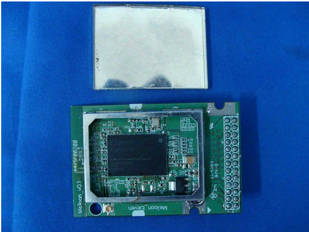
(36) EUT Photo-(5.8G)
