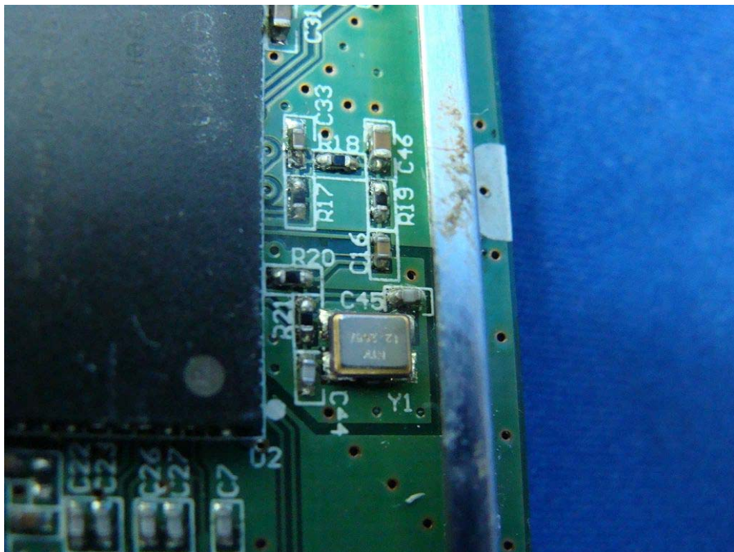
(38) EUT Photo-(5.8G)
