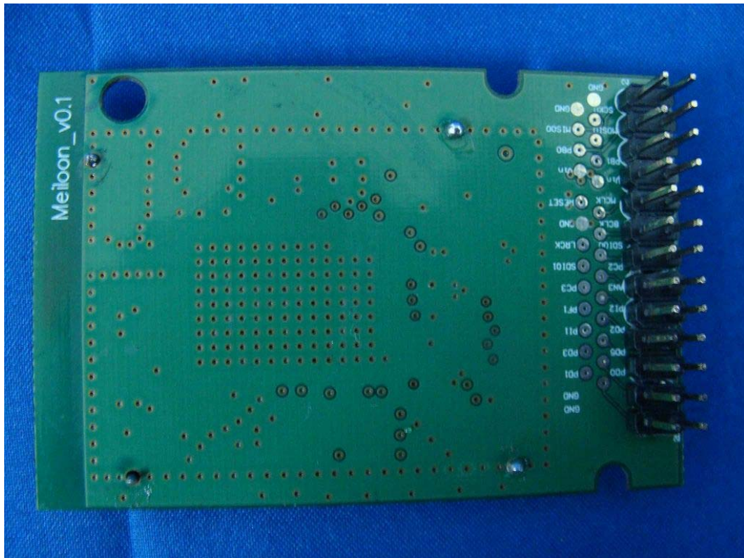
(39) EUT Photo
