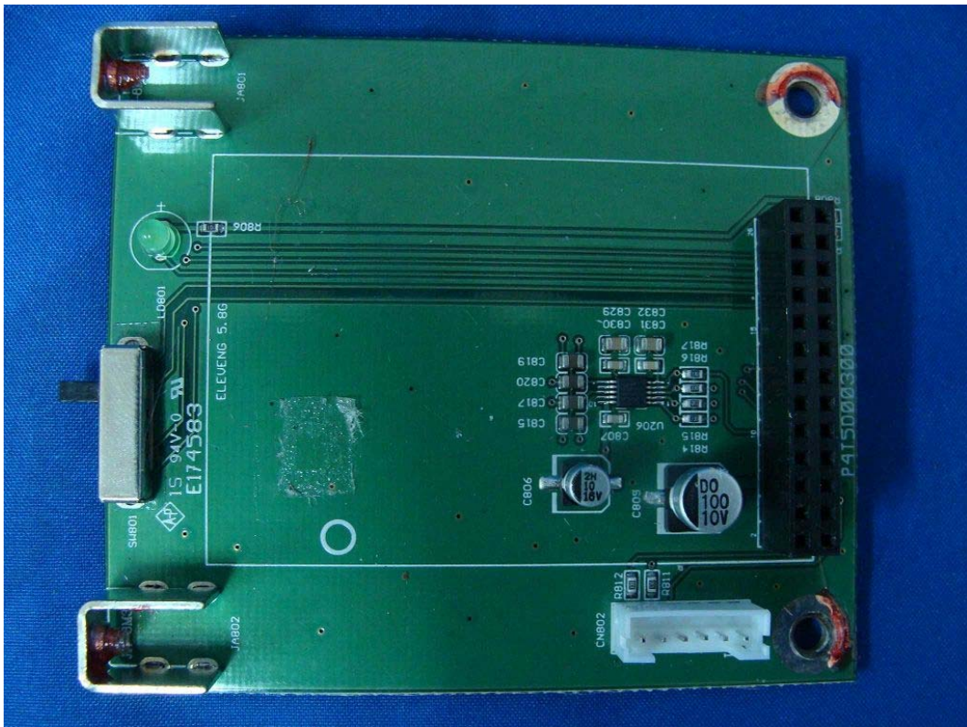
(33) EUT Photo-(5.8G)
