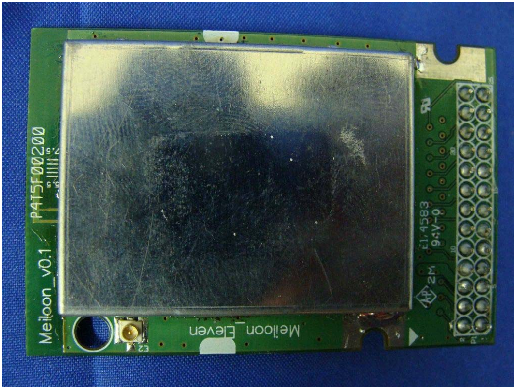
(35) EUT Photo-(5.8G)
