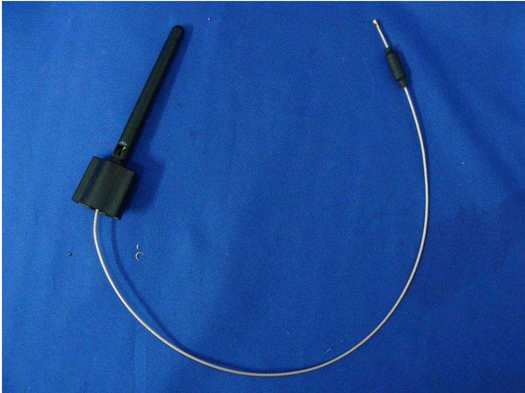
(43) EUT Photo-(5.8G)
