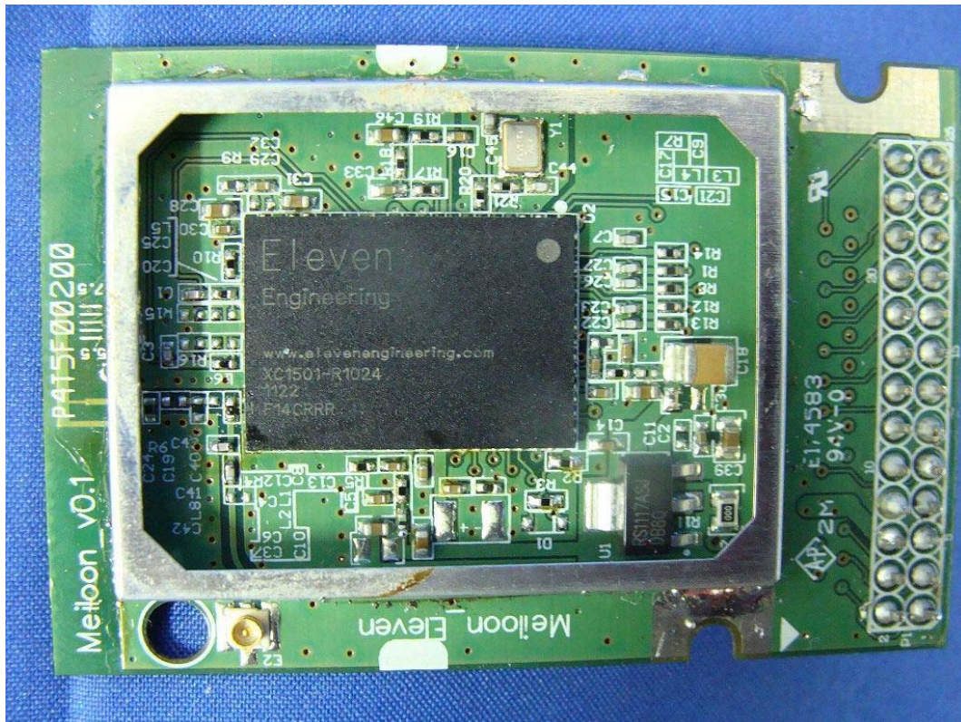
(37) EUT Photo-(5.8G)
