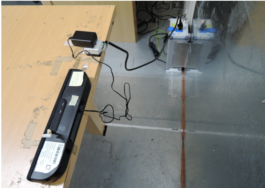
Photograph 5: Set-up for for Mains Conducted testing Back
