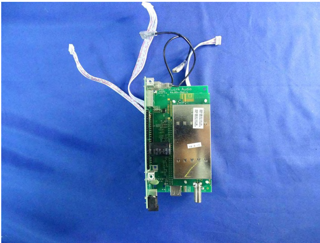
(26) EUT Photo
