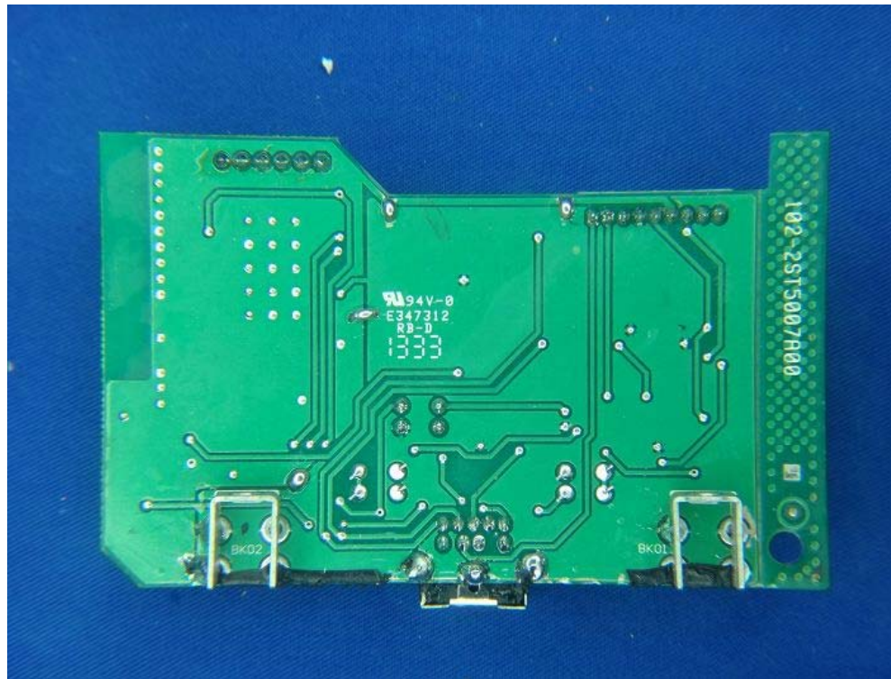
(25) EUT Photo
