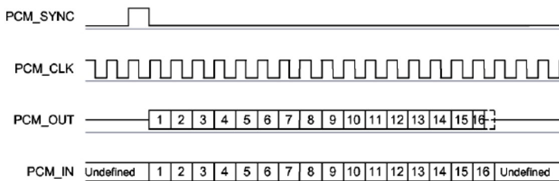
Short Frame Sync (Shown with 16-bit Sample)
