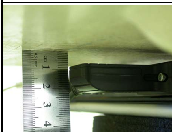
E. The bottom of the EUT face to the phantom with 9mm-separation distance.
