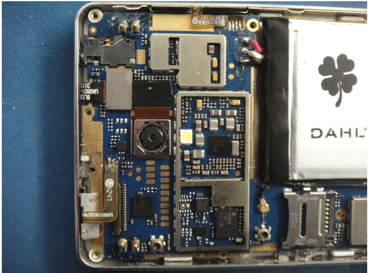
Front Main PCB Photo
