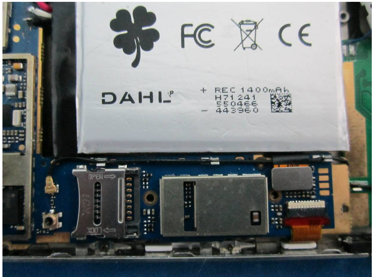
Front Main PCB Photo
