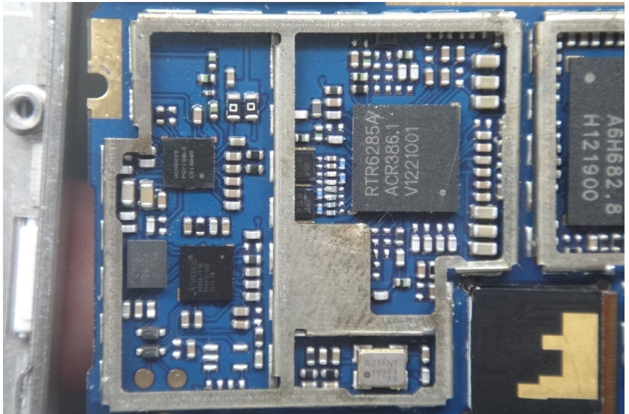
Back Main PCB Photo
