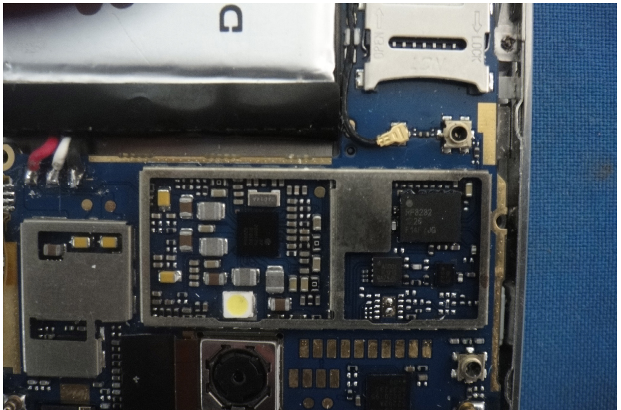
Front Main PCB Photo
