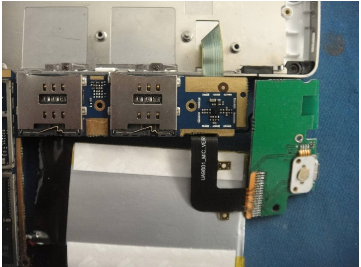
Back Main PCB Photo
