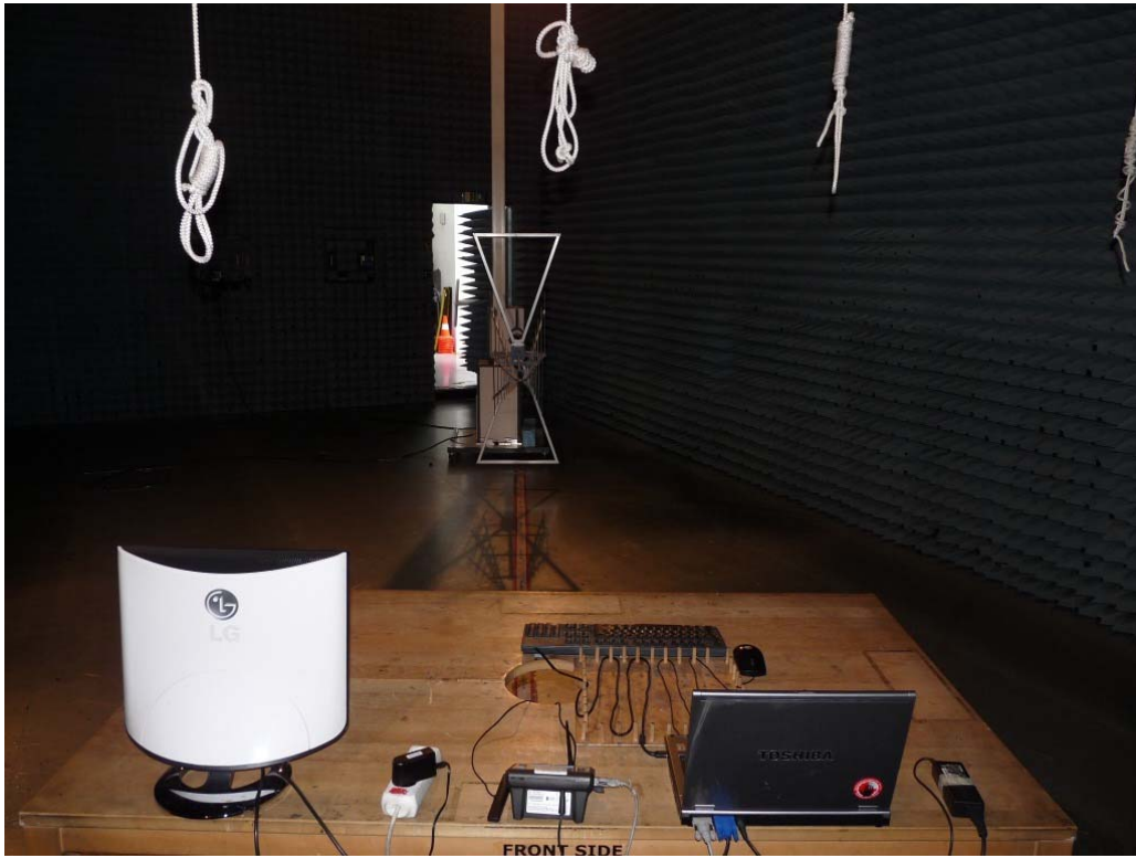
Photo 2: FCC 15B Test setup for radiated measurements (Enclosure, below 1 GHz) EUT powered by: AC/DC converter and connected to laptop computer.
