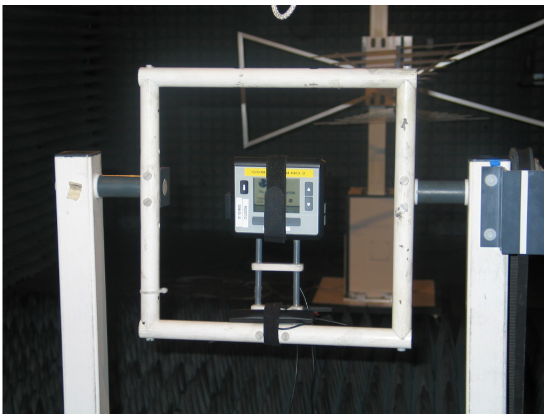
Photo 8: Test setup for the test Spurious radiated emissions above 1 GHz
