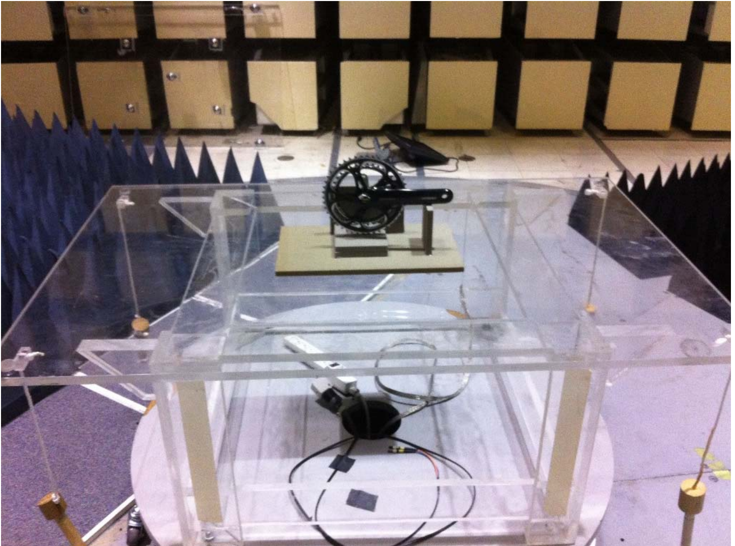
Figure 1 Radiated Spurious Emissions; Below 1 GHz
