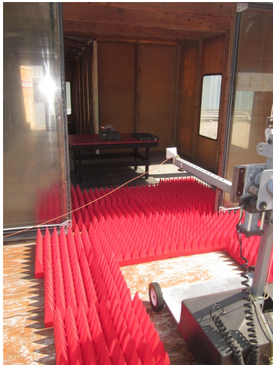
Vertical Antenna Polarization, 18 to 25 GHz
