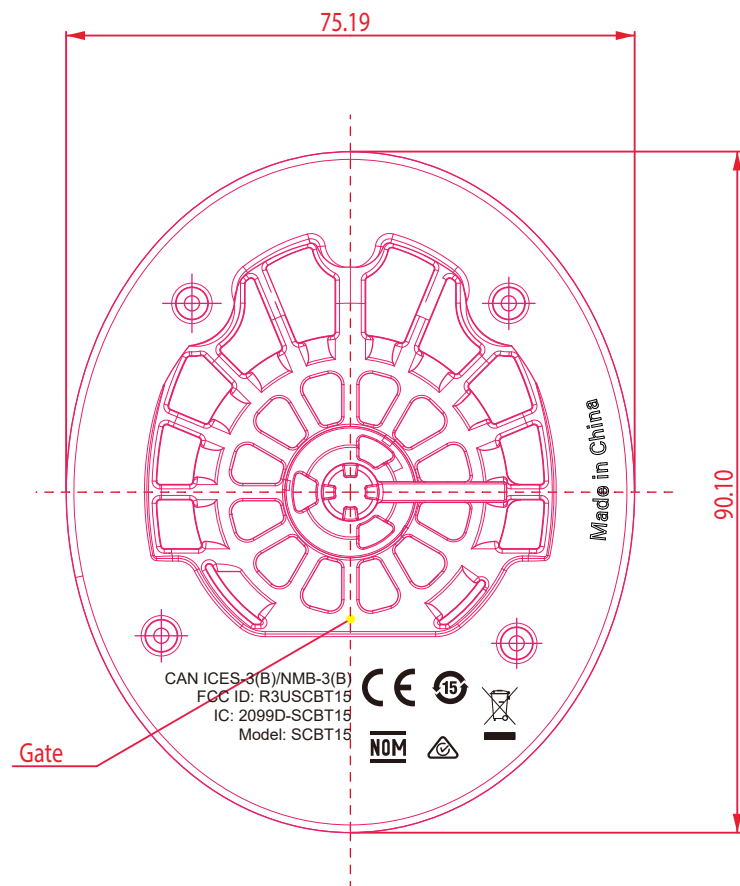
Adapt360 baffle plate L
